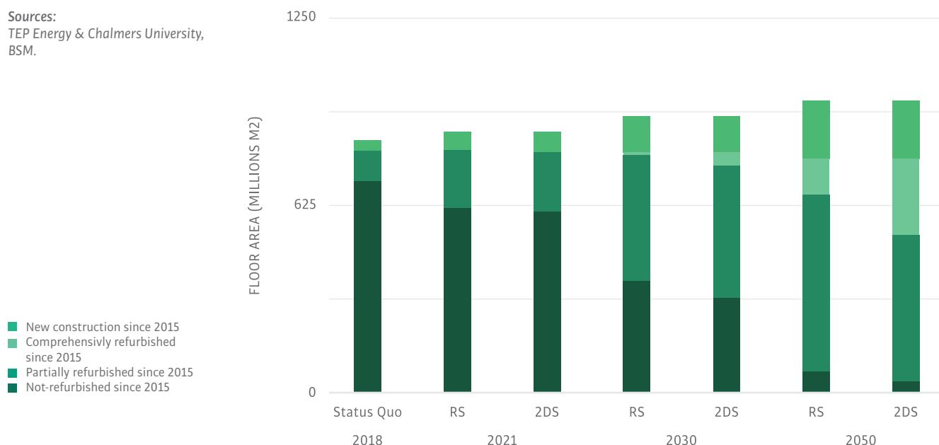
C4.1 – Refurbishment and new construction activities relating to building stock according to the Reference Scenario (RS) and the 2-Degrees Scenario (2DS).
