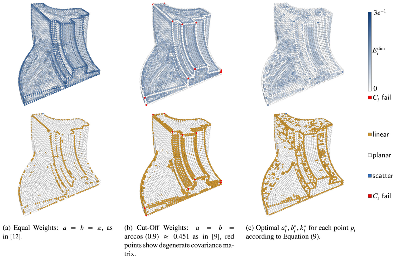
Fig. 3. The effect of the different parameters on the fandisk model. The top row shows the classification error E_i^{dim} from Eq. (7) for each point of the model, from low (white) to high error (dark blue). Note how the optimal weights from Eq. (9) have drastically reduced error in comparison to both equal weights (used by [12]) and sharp cut-off weights (used by [9]). The red points indicate elements of the point set, for which the covariance matrix from Eq. (4) degenerates given the chosen weights. Bottom row shows a feature classification according maximum value out of linearity (orange), planarity (white), and scattering (dark blue) as defined in Eq. (6). Note how equal weights fail to consistently identify edge structures. The cut-off weights manage to identify planar areas well while over-pronouncing edge structures. These are identified well by the weights from Eq. (9). (For interpretation of the references to color in this figure legend, the reader is referred to the web version of this article.)
