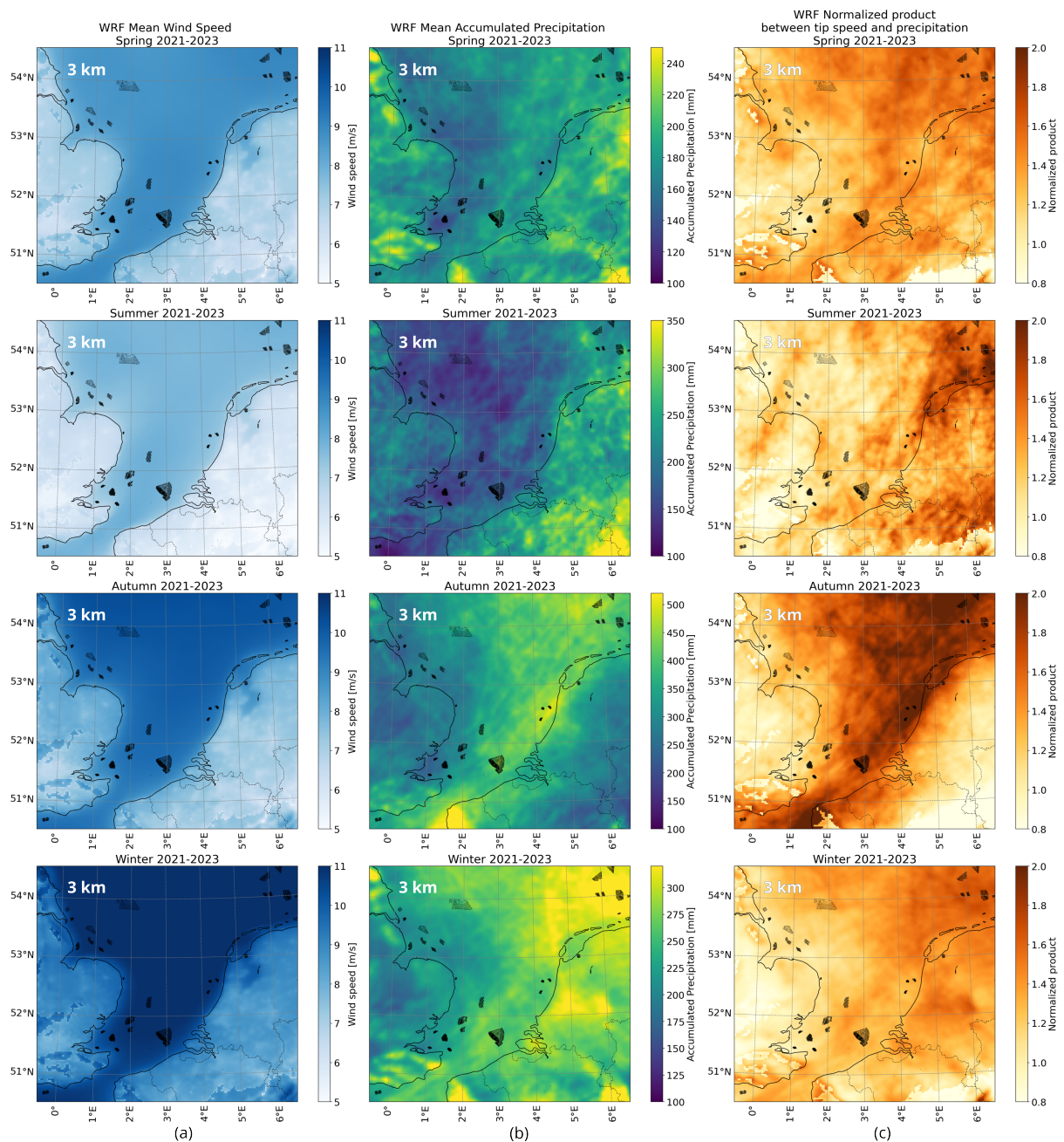
Figure 5: WRF results: (a) seasonal mean wind speed, (b) total accumulated precipitation per season, and (c) the LEE risk indicator, computed from hourly precipitation and blade tip speed.
