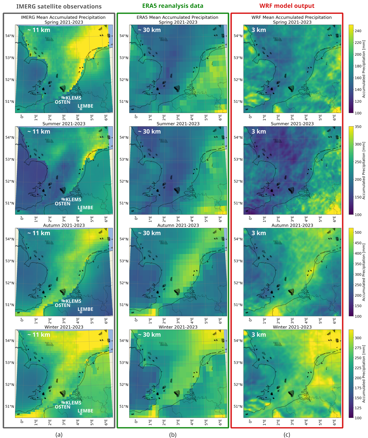
Figure 4: Seasonal precipitation maps for the Southern Bight of the North Sea: (a) IMERG satellite-based observations (~ 11 km grid), (b) ERA5 reanalysis (~ 30 km grid), and (c) WRF simulation (dynamical downscaling of ERA5 on a 3 km grid).
