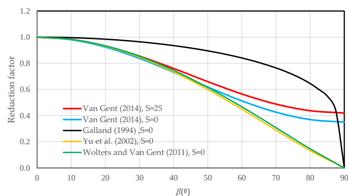
Figure 1. Comparison of methods describing the influence of oblique waves on armour size. Red and blue line: Van Gent [19], black line: Galland [13], yellow line: Yu et al. [17] and green line: Wolters and Van Gent [19].
