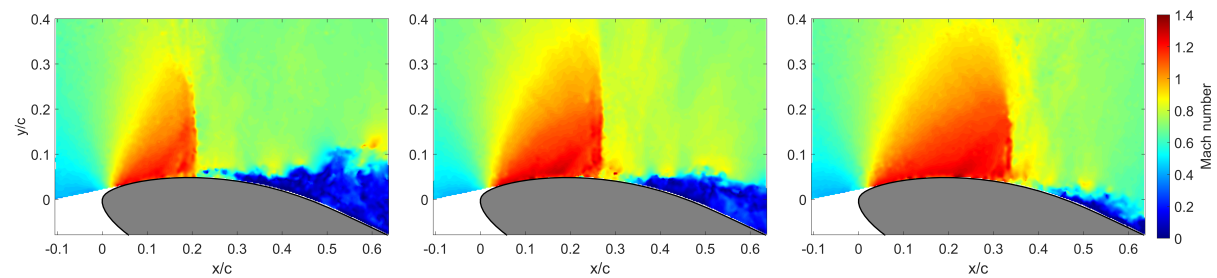
Figure 12: Instantaneous frames for Ma_\infty = 0.6 , AoA = -10^\circ showing the appearance of a moving shock wave at different streamwise locations over the airfoil.
