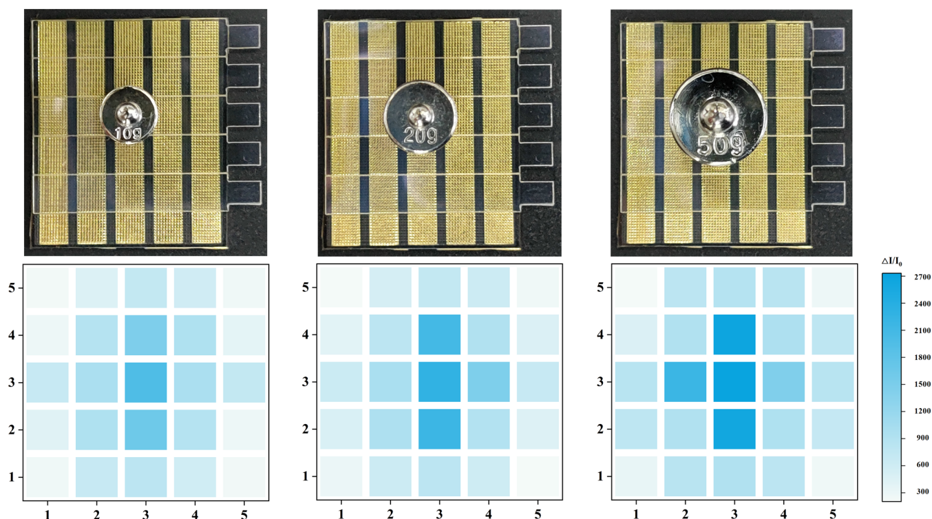
Figure 7. Real-time detection of spatial pressure distribution capabilities on a 5 × 5 sensor array using weights of different masses (10, 20, and 50 g).
