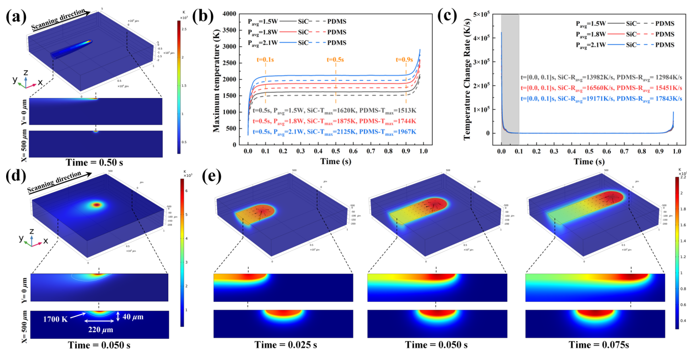
Figure 3. (a) 3D and cross-sectional isothermal surface distributions of PDMS and SiC during CLP reaction ( P_{avg} = 1.5 W, v_{ss} = 10 mm/s, and time = 0.5 s). (b) and (c) Maximum temperature and maximum temperature change rate curves of PDMS and SiC with time under different laser average powers (1.5, 1.8, and 2.1 W). (d) 3D and cross-sectional temperature distributions of PDMS and SiC during ILP reaction (time = 0.050 s). (e) 3D and cross-sectional temperature evolution distributions of the PDMS and SiC during CLP reaction (time = 0.025, 0.050, and 0.075 s).
