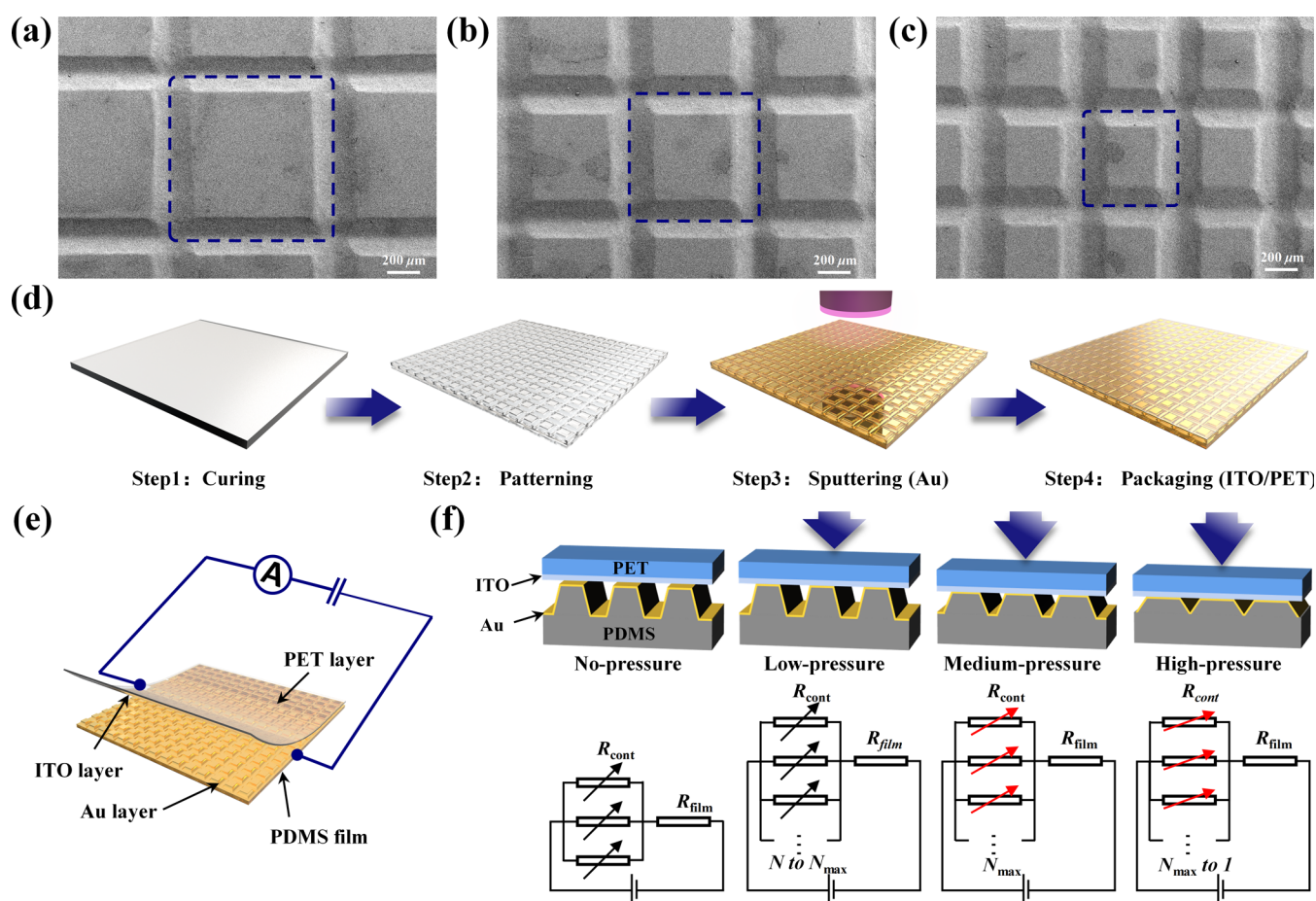
Figure 4. (a)–(c) Surface topography of PDMS micro-truncated pyramid arrays with different scanning pitches (#12 × 12, #16 × 16, and #20 × 20) fabricated using continuous laser direct writing technology. (d) Schematic illustration of the fabrication process for flexible pressure sensors with micro-truncated pyramid array structure. (e) Simplified circuit schematic for testing the performance of the flexible pressure sensor. (f) 3D cross-sectional schematics and equivalent circuit diagrams of the sensor under different pressure conditions.
