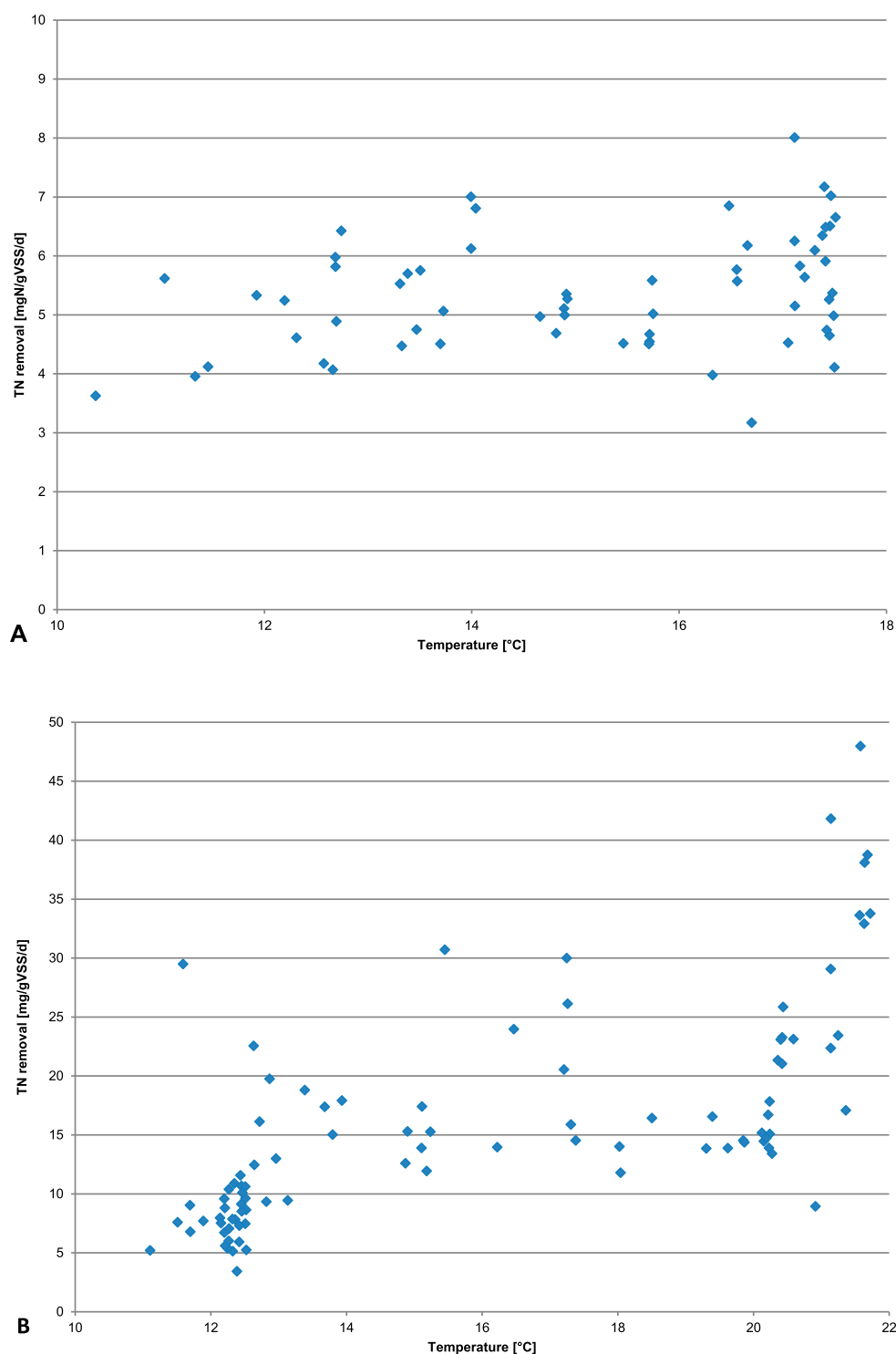
Figure 2. Effect of temperature on the total nitrogen removal, in A: period 3 and B: period 4. Average BOD/N ratio of period 3 was 1.2 \pm 0.4 and 2.5 \pm 1.8 for period 4.
