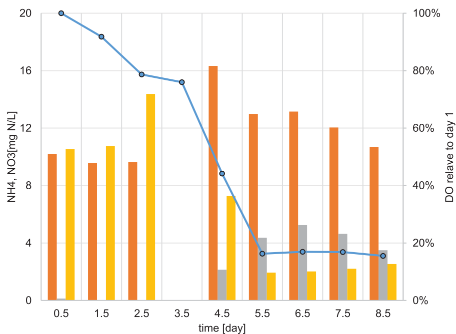
Figure 5. Influent and effluent of the reactor with different oxygen concentrations (data are 24 h averaged values), temperature is constant at 24°C. Influent ammonium in orange (first) bars, effluent ammonium in grey (second) bars, effluent nitrate in yellow (third) bar and relative DO in blue line (colour online only).
