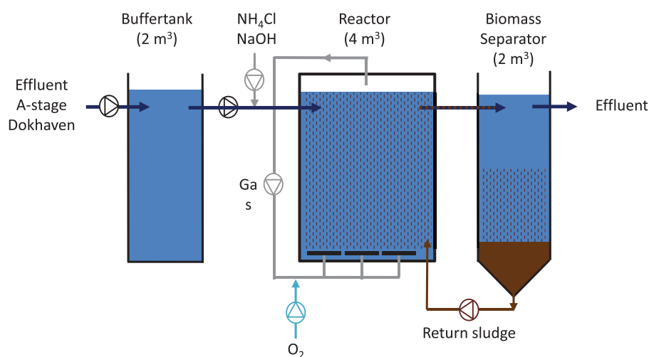
Figure 1. Schematic representation of the lay-out of the PN/A reactor.
