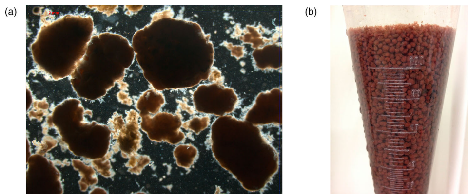
Figure 3. Granules in the inoculum of the PN/A reactor at the beginning of period 2.
