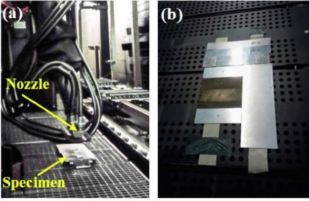
Fig. 3. The shot peening forming process of FMLs: (a) the objective graph; (b) specimens to be processed.
