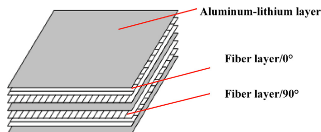
Fig. 1. The FMLs studied constitute an FML3-3/2-0.3 lay-up.
