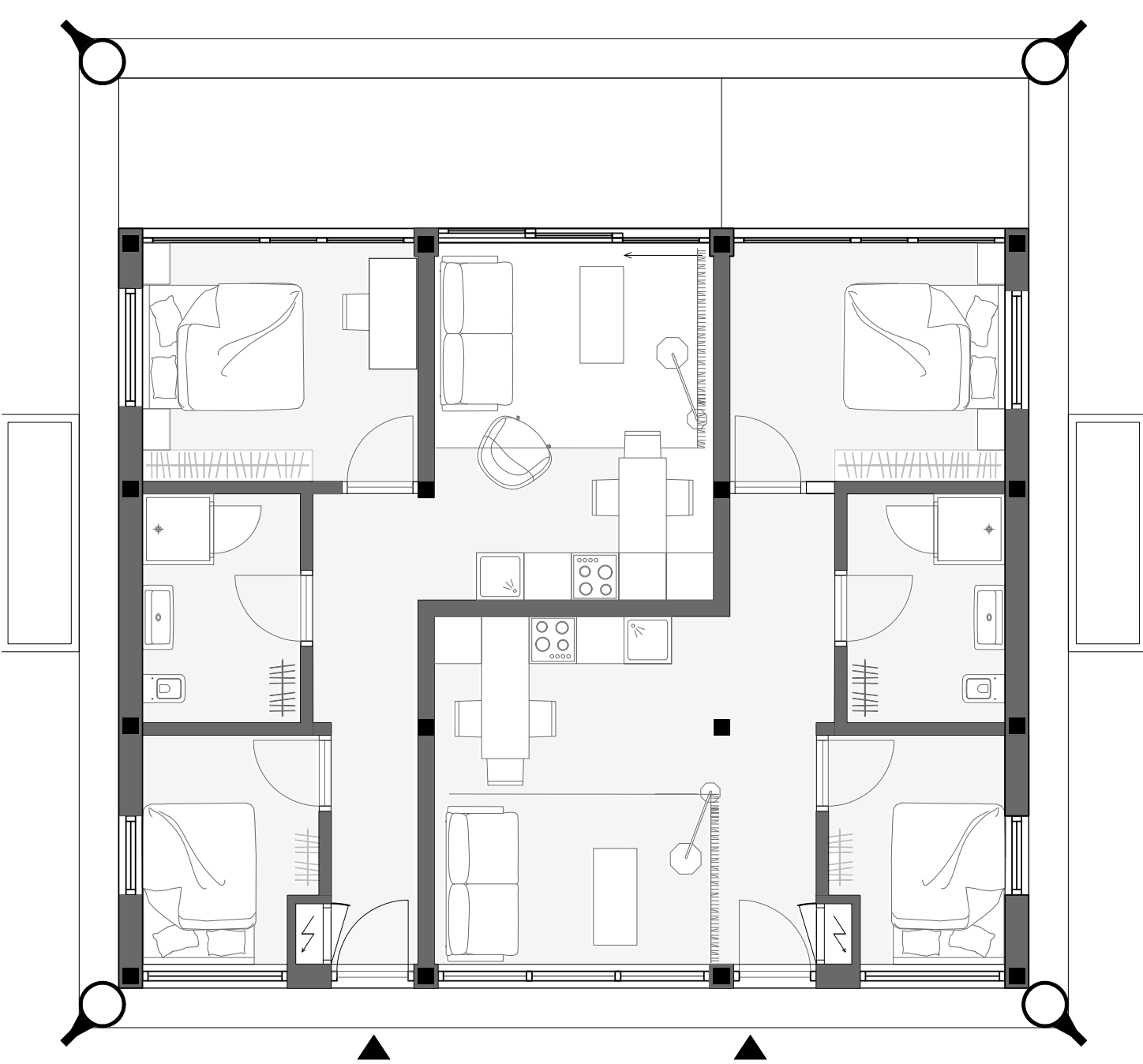
Friends apartment 50 m2
