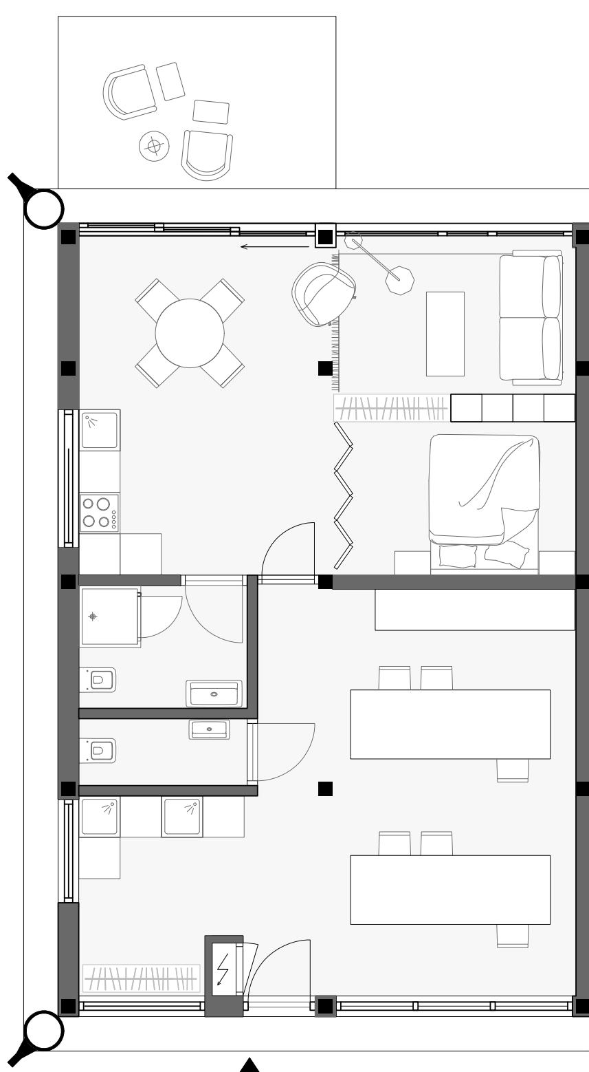
Creative apartment 78 m2
