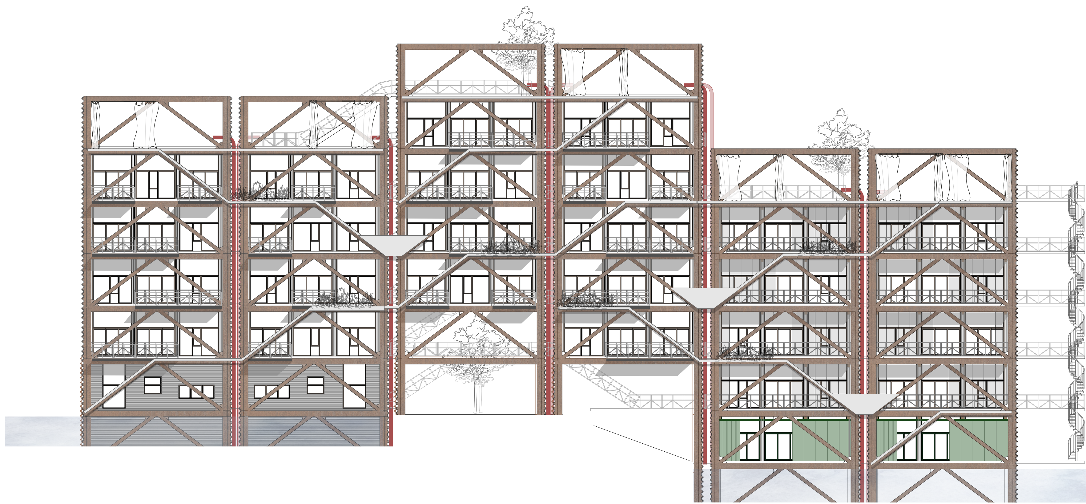
North facade 1:200
