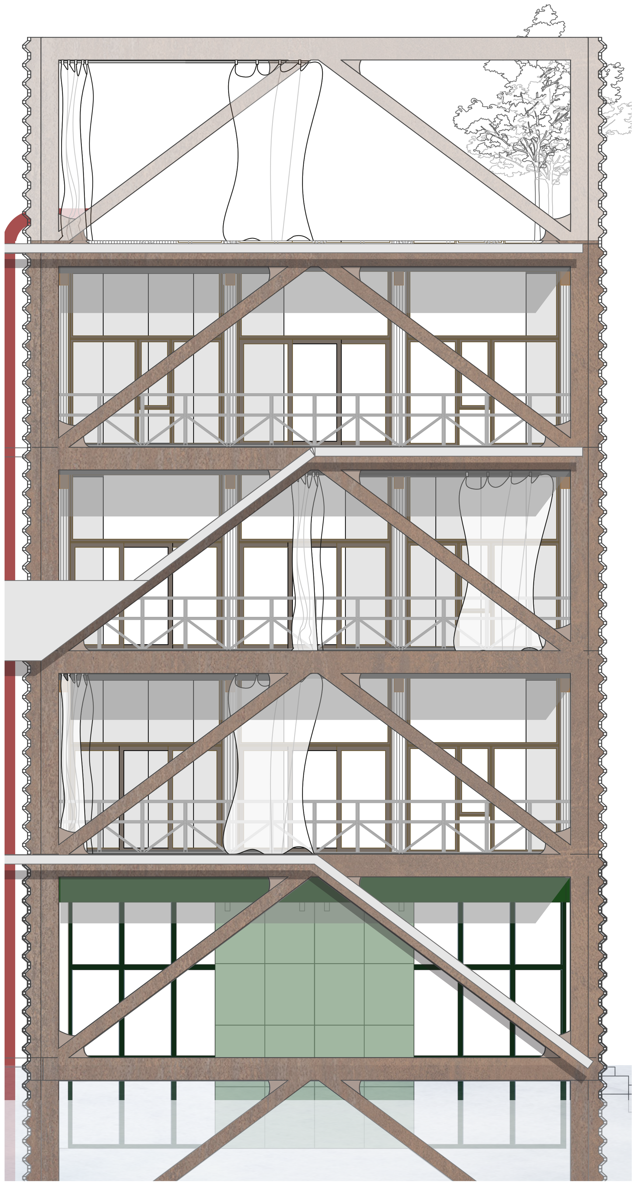
Facade Fragment 1:20
