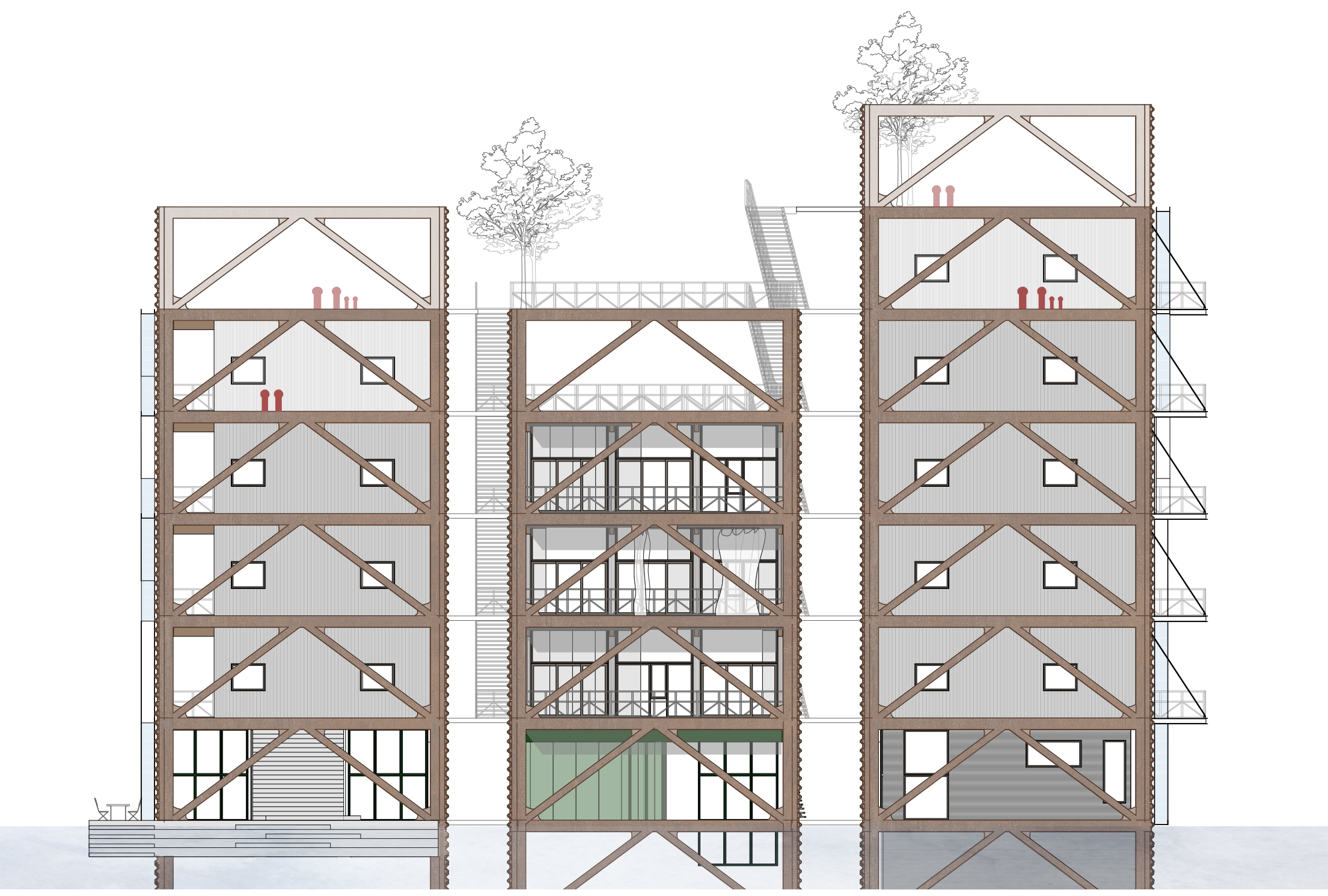
East facade 1:200
