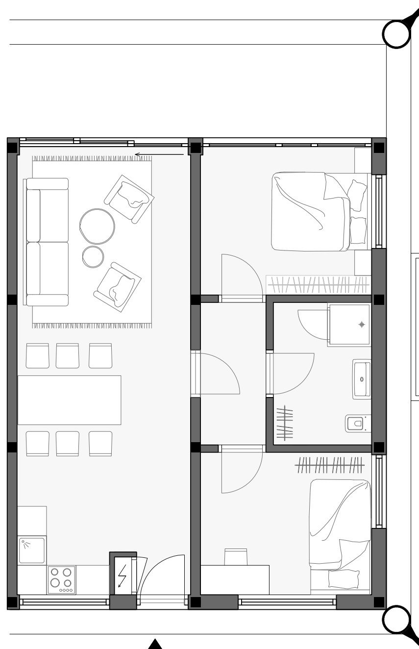
Starter apartment 66 m2
