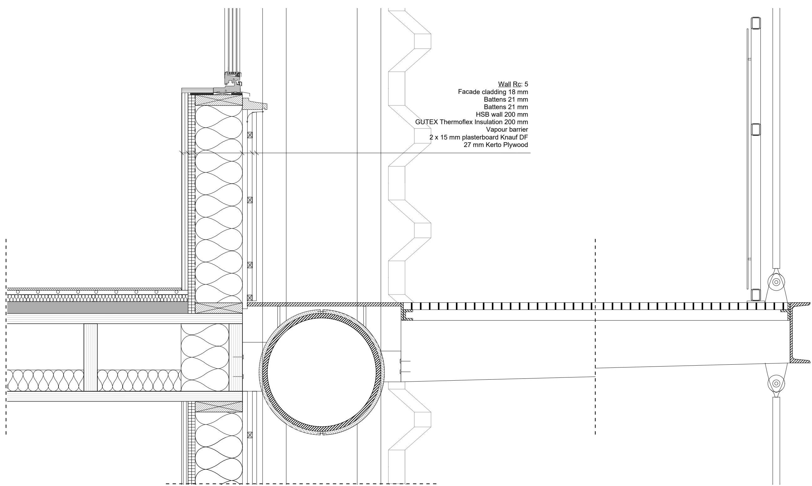
Floor Detail 1:5
