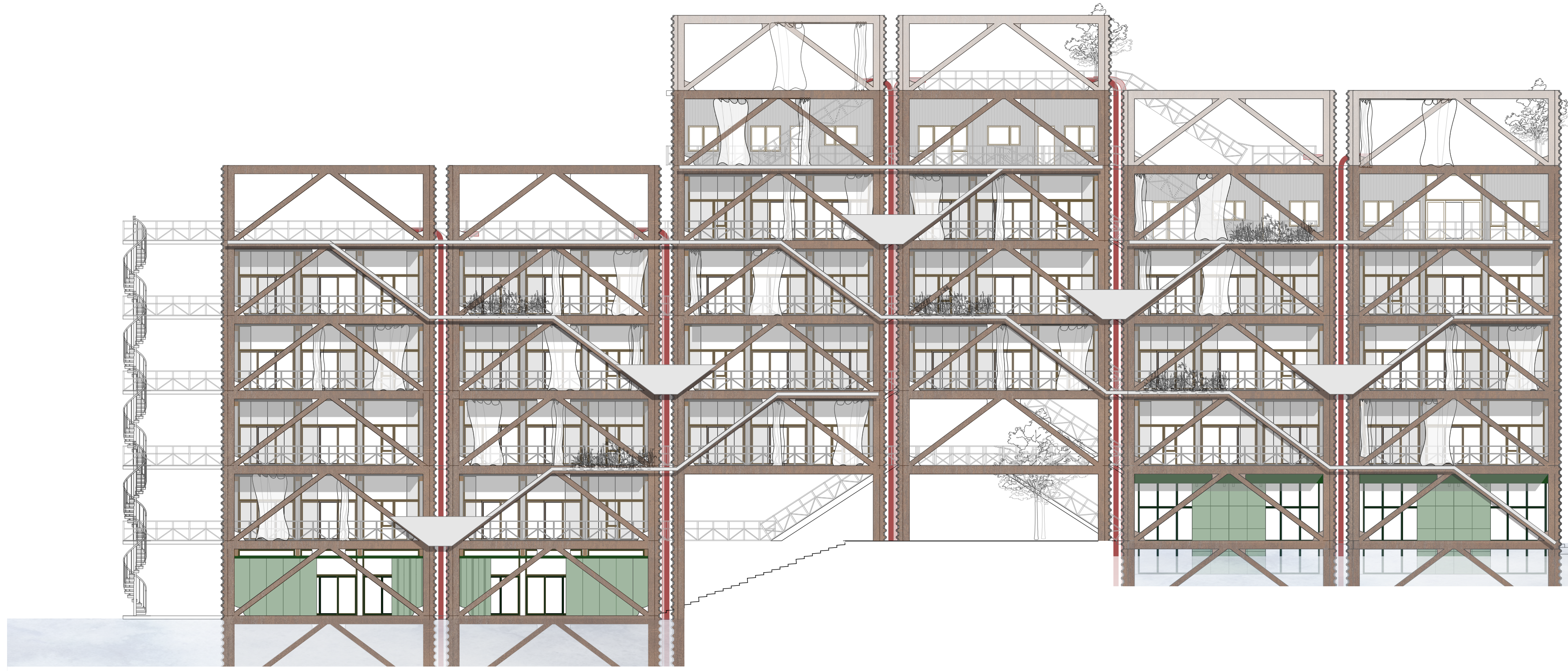
South facade 1:200
