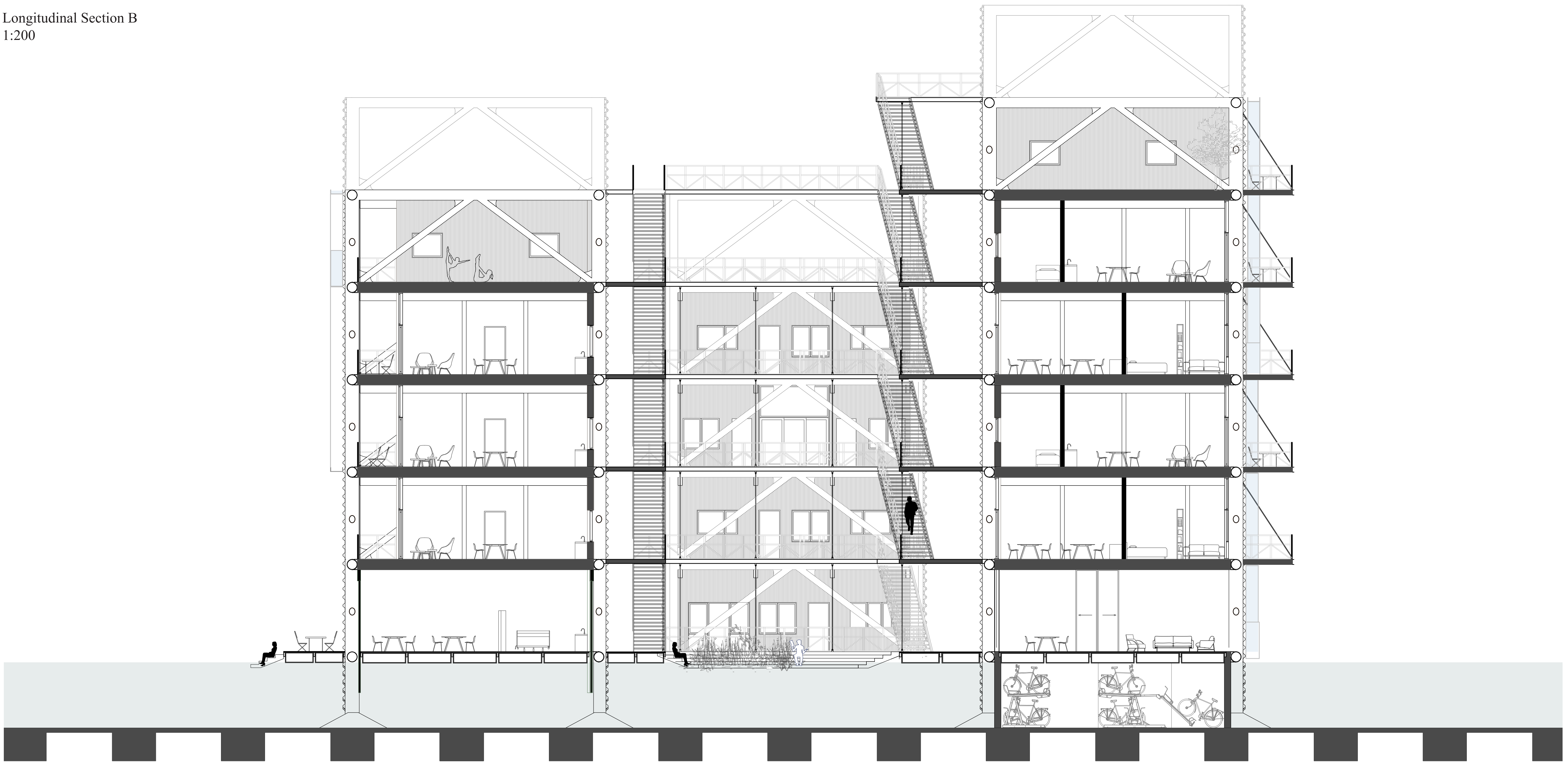
Cross Section C 1:100
