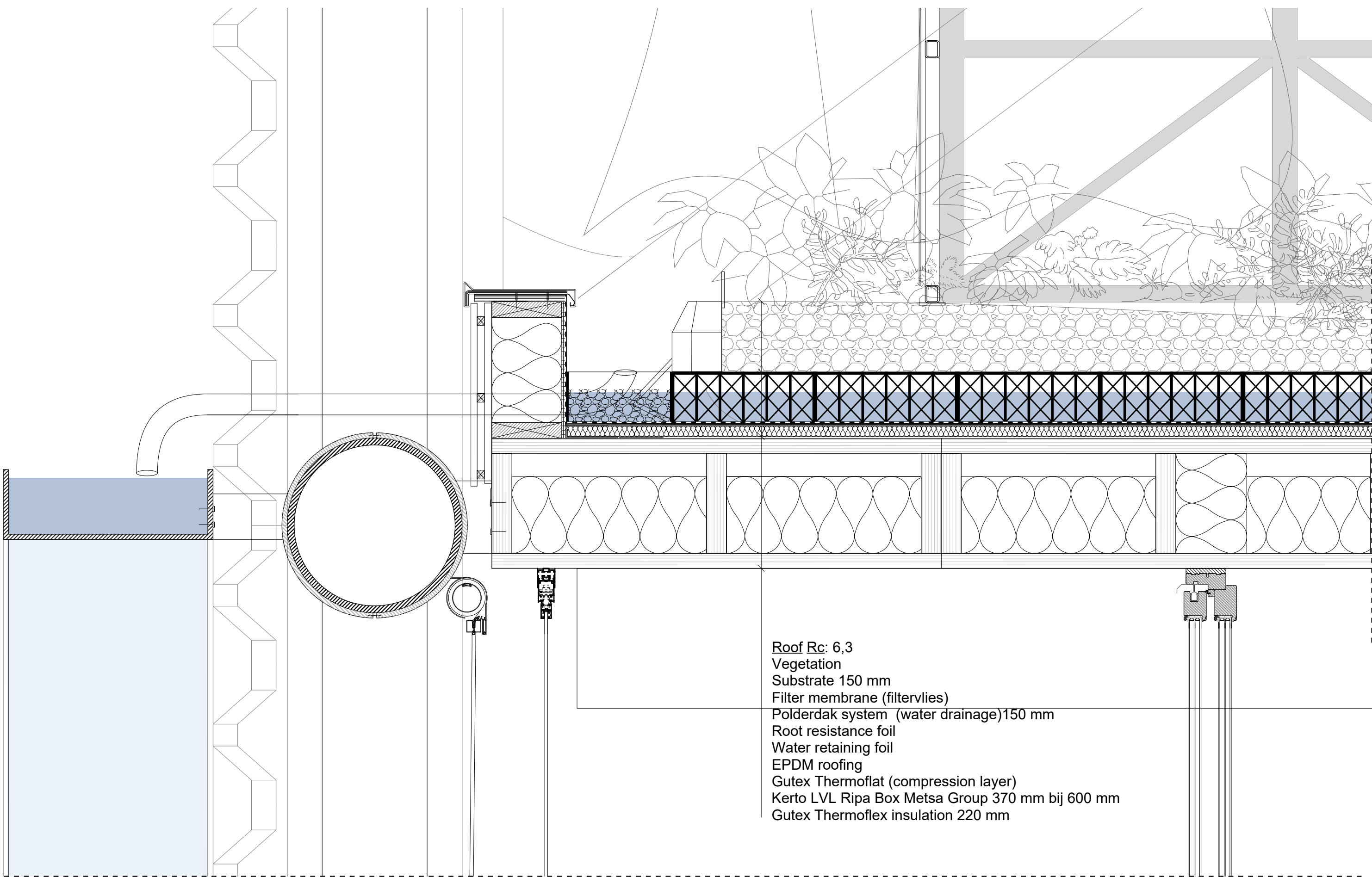
Roof Detail 1:5
