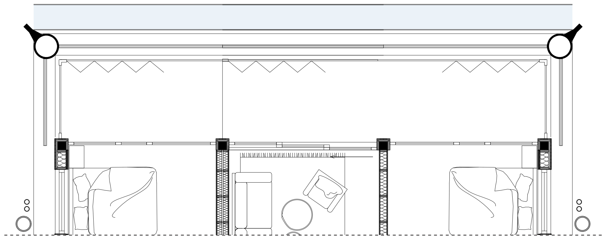
Facade Fragment floating 1:20
