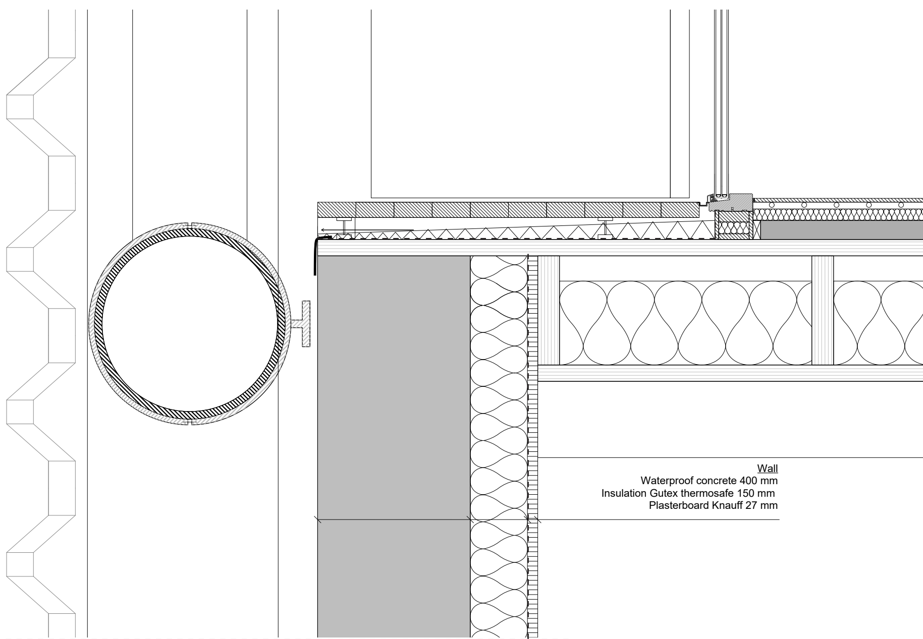
Floating Detail 1:5
