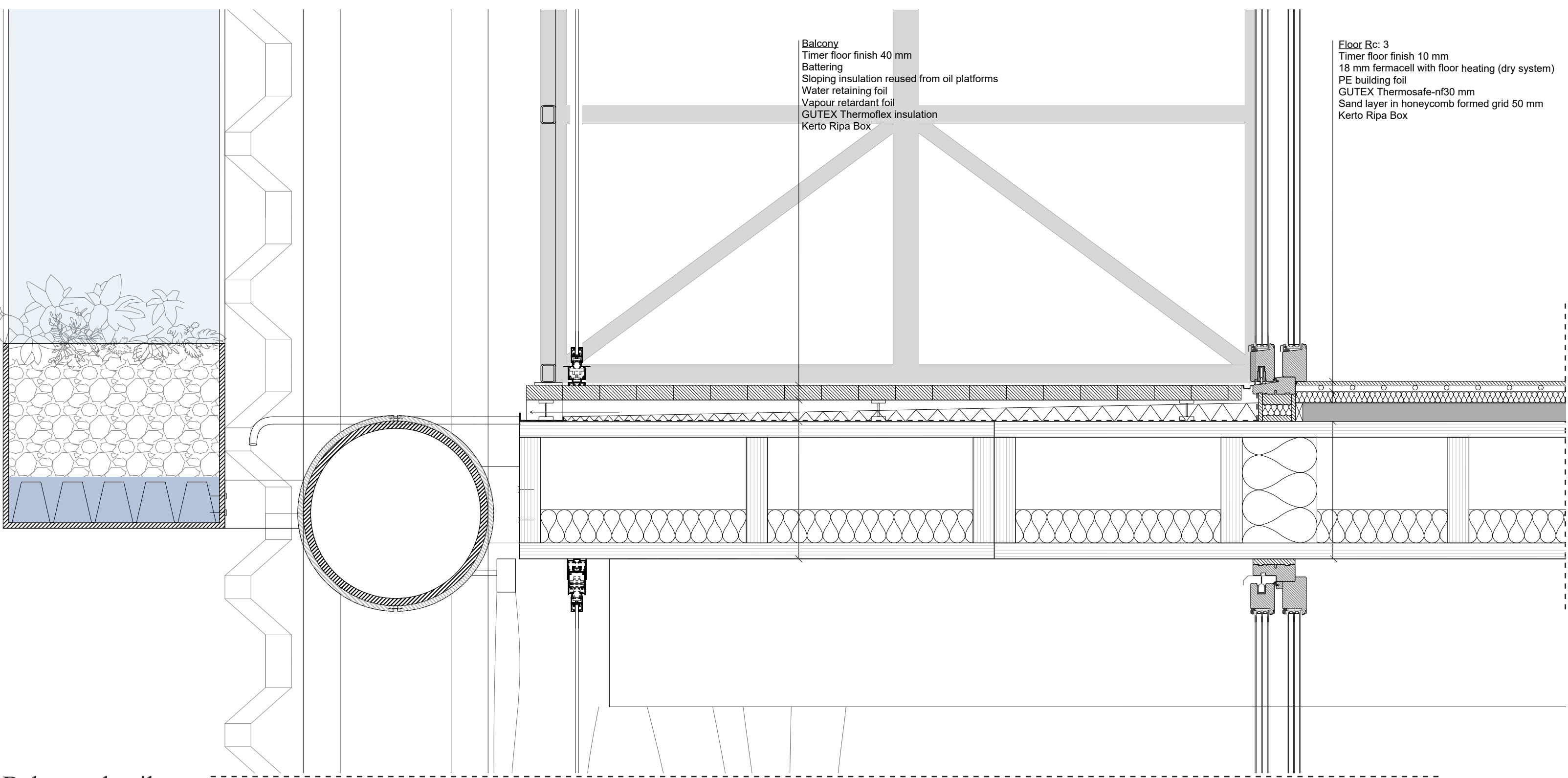
Balcony detail 1:5
