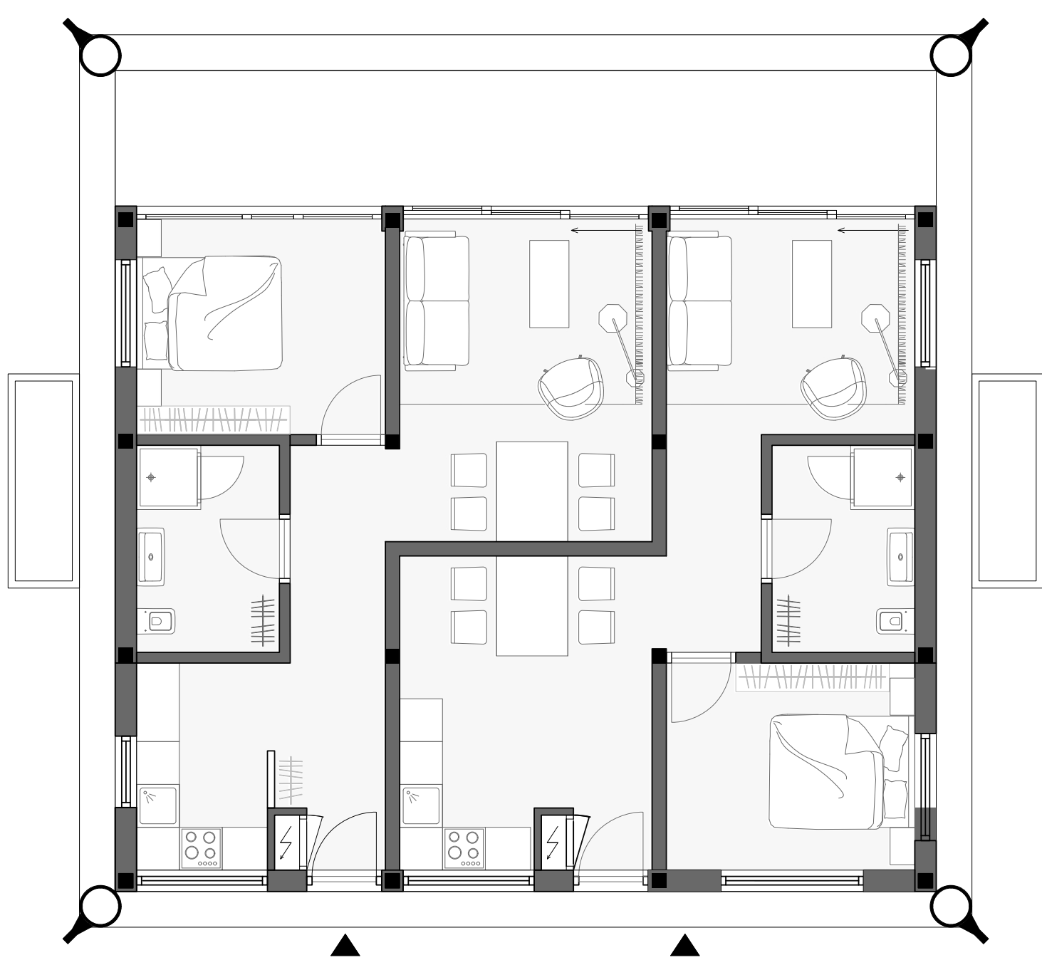
Elderly apartment 50 m2
