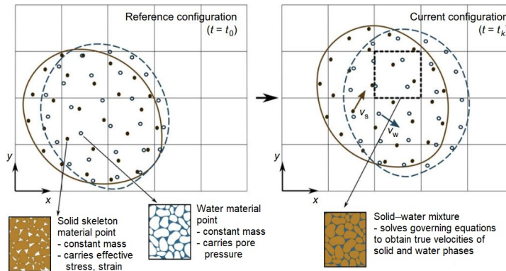
Figure 2.9: Coupled MPM implementation using two sets of MPs to describe the response of both phases (Soga et al. , 2015)
