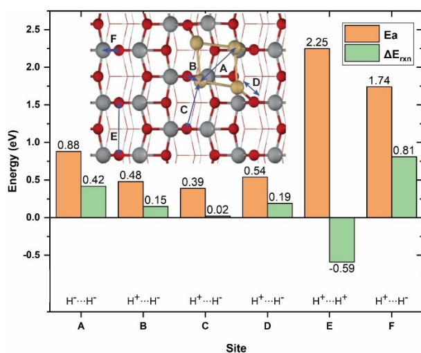
Figure 2. Activation energy ( E_a ) and reaction energy ( \Delta E_{\text{rxn}} ) for \text{H}_2 dissociation at all possible active sites of \text{Cd}_4/\text{TiO}_2 catalyst.
