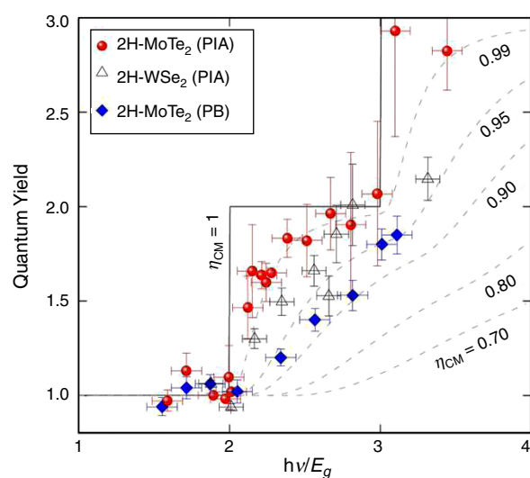
FIG. 17. CM QY vs bandgap multiple in \text{MoTe}_2 and \text{WSe}_2 . 51 J.-H. Kim, M. R. Bergren, J. C. Park, S. Adhikari, M. Lorke, T. Frauenheim, D.-H. Choe, B. Kim, H. Choi, T. Gregorkiewicz, and Y. H. Lee, Nat. Commun. 10 , 5488 (2019); licensed under a Creative Commons Attribution (CC BY) license.
