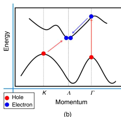
FIG. 16. (a) Maximum THz conductivity vs bandgap multiple in \text{MoTe}_2 showing CM threshold around three times the bandgap. (b) Schematic of asymmetric excitation in \text{MoTe}_2 . 52 With kind permission from the ACS. The original article can be found at https://pubs.acs.org/doi/10.1021/acs.nanolett.0c01693 . Further permissions related to the material excerpted should be directed to the ACS.
