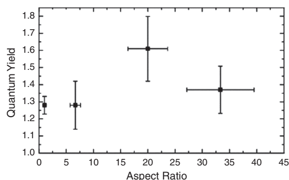
FIG. 12. CM QY at 3.86 eV photoexcitation for Si QDs (aspect ratio 1, the first data point) and Si NRs with different aspect ratios. 36 Reprinted with permission from C. J. Stolle, X. Lu, Y. Yu, R. D. Schaller, and B. A. Korgel, Nano Lett. 17 , 5580 (2017). Copyright 2017 American Chemical Society.
