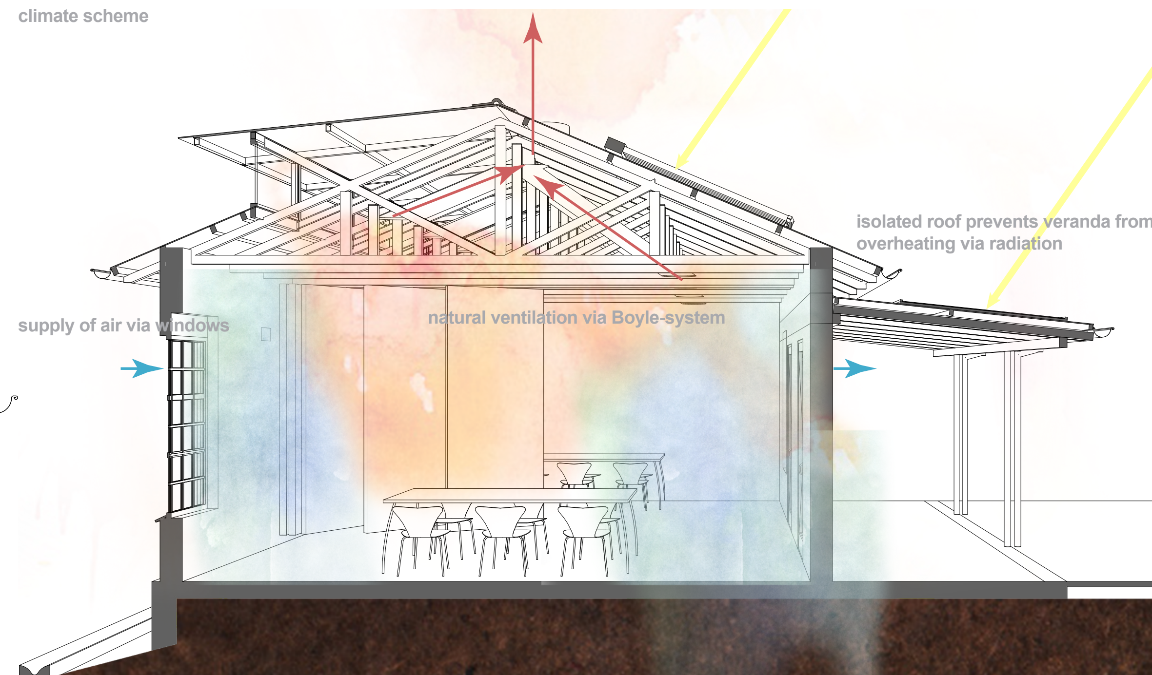
climate scheme
