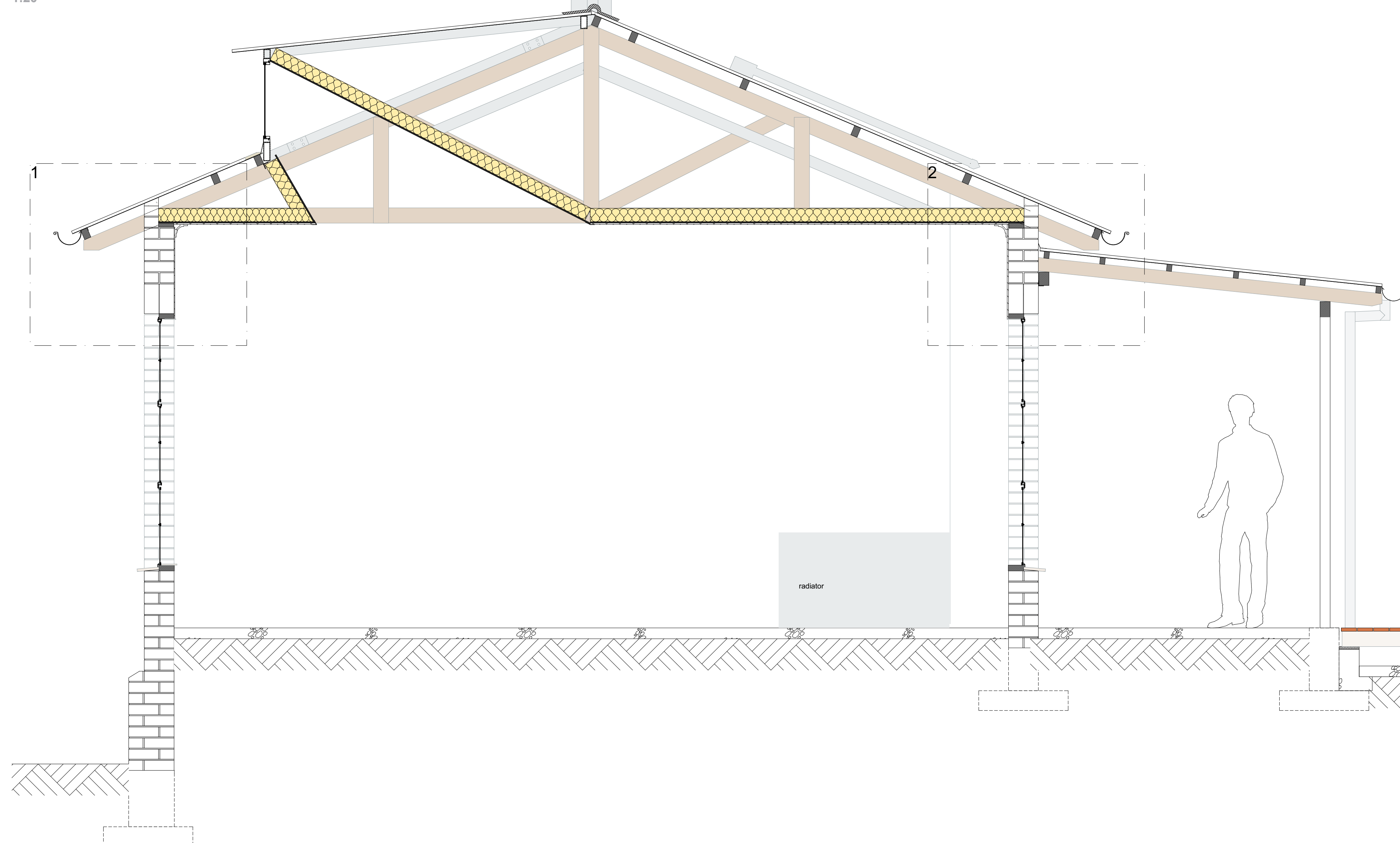
section 1:20
