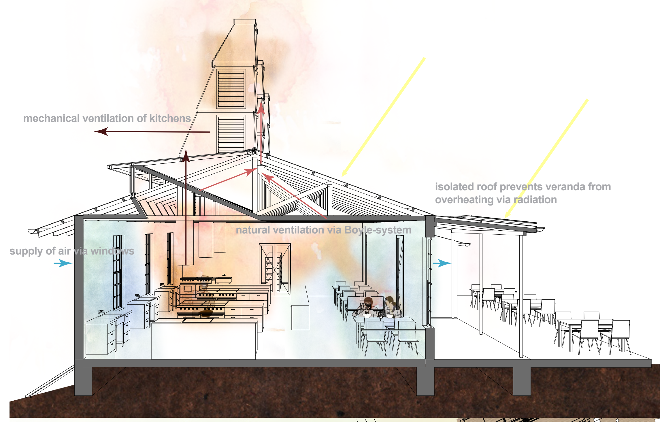
ventilation scheme
