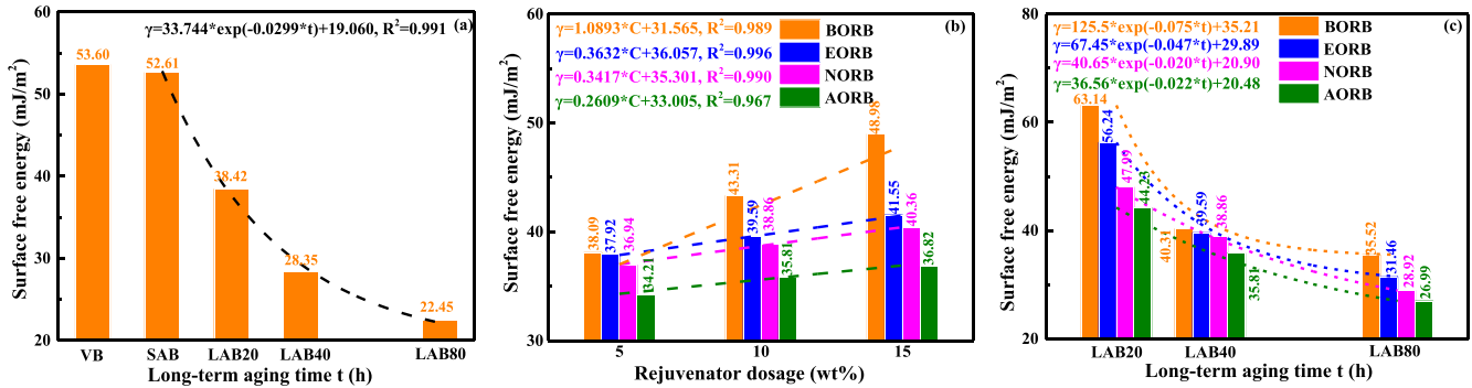
Fig. 21. Surface free energy \gamma of the virgin, aged, and rejuvenated bitumen.
