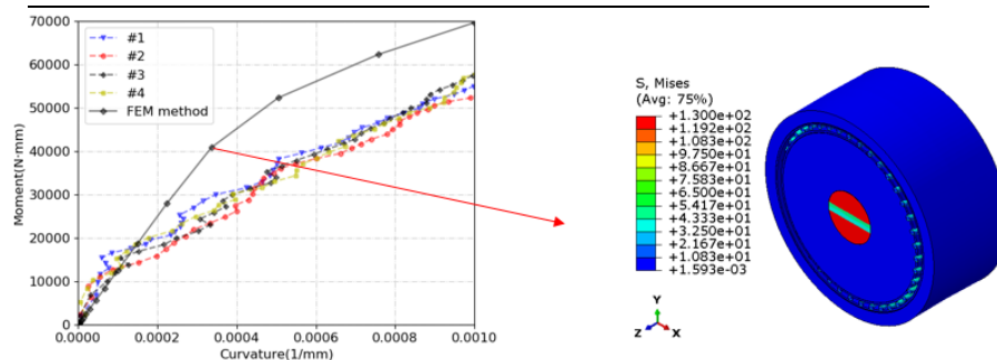
Fig. 10 Curvature-moment from FEM method and test results
