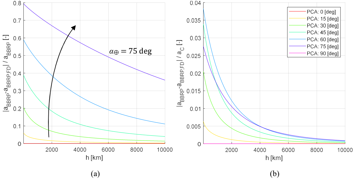
Figure 7. Relative error (left) and absolute error (adimensionalized with respect to the solar-sail characteristic acceleration, right) between the BBRP accelerations of the spherical and FD models. The PCA increases in the direction of the arrow.
