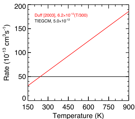
Figure 5. Reaction rates for the \text{N}(^2\text{D}) + \text{O}_2 \rightarrow \text{NO} + \text{O} reaction used in TIEGCM (black) and proposed by Duff et al. [2003] (red).
