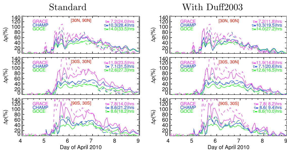
Figure 8. Percentage changes of orbit-mean neutral density along GOCE (green), CHAMP (blue), and GRACE (magenta) trajectories in the latitudinal regions of (top row) 30^{\circ}\text{N} – 90^{\circ}\text{N} , (middle row) 30^{\circ}\text{S} – 30^{\circ}\text{N} , and (bottom row) 30^{\circ}\text{S} – 90^{\circ}\text{S} . Observations are shown by dashed lines and simulations by solid lines. Comparisons between observations and the standard TIEGCM run are shown on the left, and comparisons between observations and the modified run with the reaction rate (M4) from Duff et al. [2003] on the right. The parameter \tau denotes the e -folding recovery time, with the value outside (inside) the parenthesis being derived from observations (simulations).
