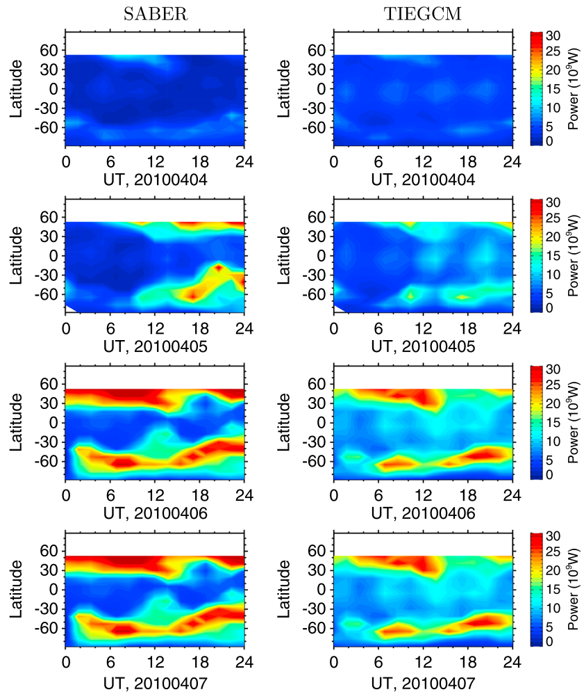
Figure 3. NO cooling power along TIMED trajectory from (left column) SABER measurements and (right column) TIEGCM simulations. The SABER instrument is in the “southward” viewing mode, so there are no observations beyond \sim 55^\circ\text{N} .
