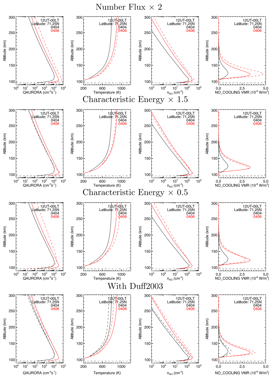
Figure 4. Comparisons of the ionization rate (QAUORA) due to particle precipitation, neutral temperature, NO number density, and NO cooling rate at 71.25°N at midnight (00:00 LT) between a standard TIEGCM run and a modified run. Profiles on the quiet day (12:00 UT on April 4) are plotted out in black, and profiles on the storm day (12:00 UT on 6 April) in red. Profiles from the standard TIEGCM run are plotted using solid lines and are unchanged between rows, while the row-dependent profiles from each modified run are plotted using dashed lines. From top to bottom, it shows the comparisons between the standard TIEGCM run with (first row) M1, (second row) M2, (third row) M3, and (fourth row) M4.
