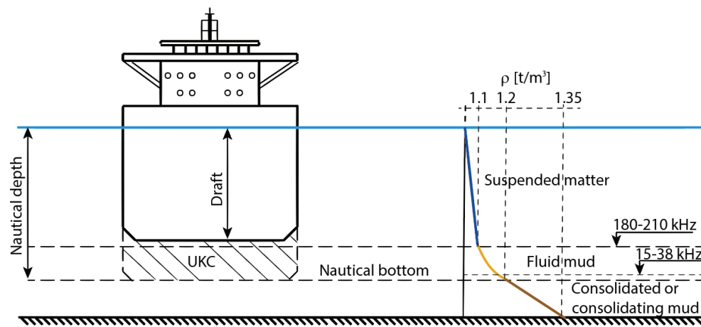
Figure 2. The nautical bottom concept at the density limit of 1.2 t/m 3 . (From Kirichek et al., 2018)
