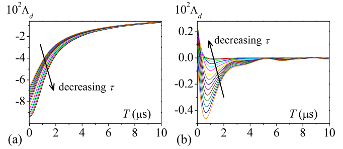
FIG. 8. Plots of the amplitude \Lambda_d(\tau_n, T) vs T at fixed \tau_n = (\pi/\omega_I)n , for (a) odd n = 1, 3, \dots, 29 , and (b) even n = 2, 4, \dots, 30 . The plots demonstrate the reduction of \Lambda_d(\tau_n, T) when going from odd to even n . For small n , the decrease of \Lambda_d(\tau_n, T) from odd to even n is more than two orders of magnitude. For large n , it is more than 15 times.
