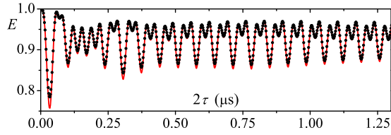
FIG. 7. Comparison of the polymer chain orientation disorder averaged exact relation Eq. (10) (black points) and approximation Eq. (A4) (red line).
