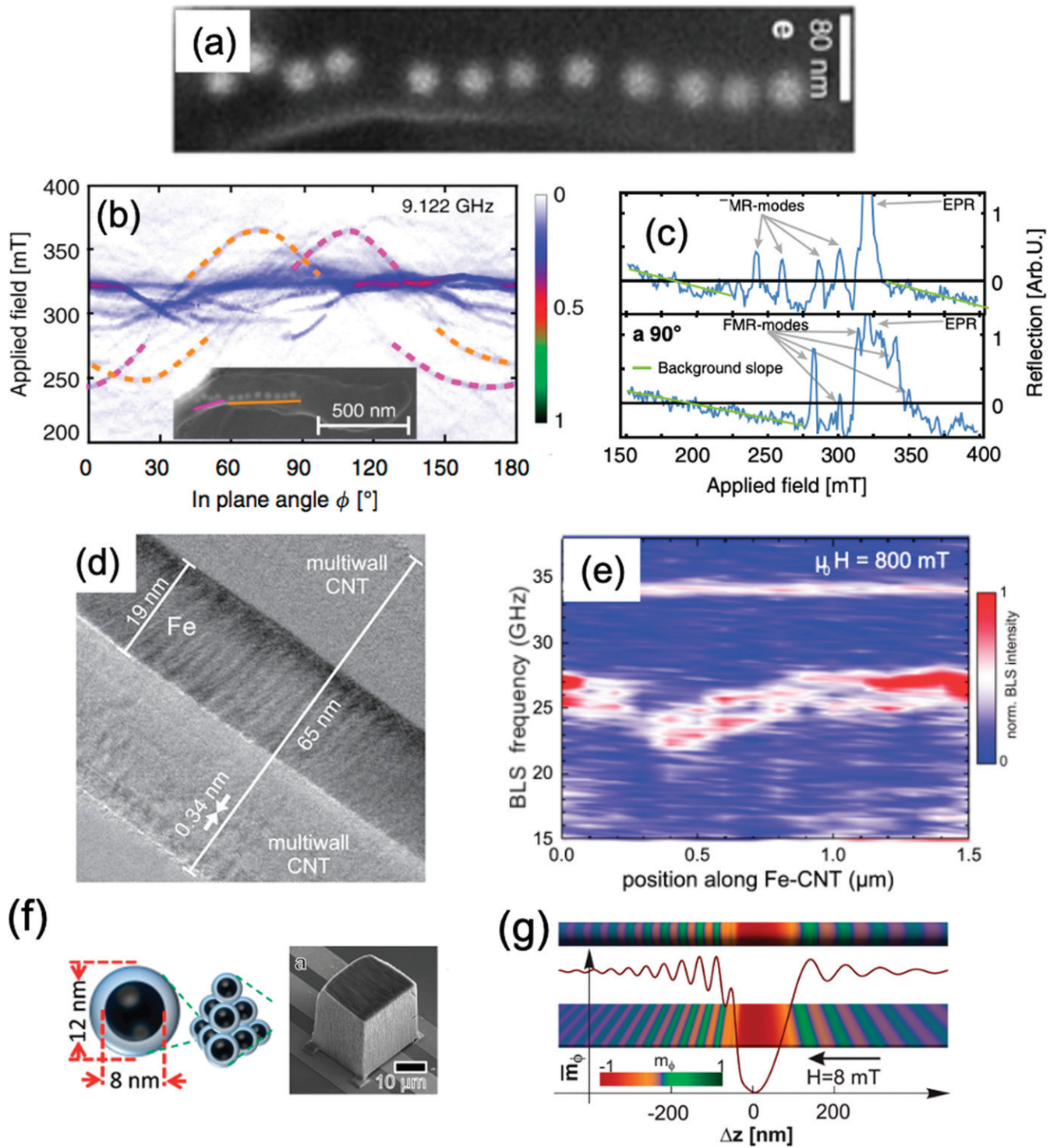
Figure 3. (a) Magnetite crystal chain grown by magnetotactic bacteria. (b) Angular dependence of magnetite crystal chain FMR spectra and (c) two single spectra recorded at 0° and 90°. (a-c) Reproduced from [25]. CC BY 4.0. (d) TEM of a single Fe filled carbon nanotube suspended across micro-resonator. (e) Thermal spin-wave spectrum of FeCNT obtained using BLS. (d), (e) Reproduced from [26]. CC BY 4.0. (f) Schematic of \text{Fe}_3\text{O}_4 crystal monomer (left), crystals (middle) and an SEM of the machined \text{Fe}_3\text{O}_4 crystal upon a CPW. Reproduced from [27]. © IOP Publishing Ltd. All rights reserved.. (g) Spin-Cherenkov effect in magnetic nanotube. Reprinted from [28], with the permission of AIP Publishing.
