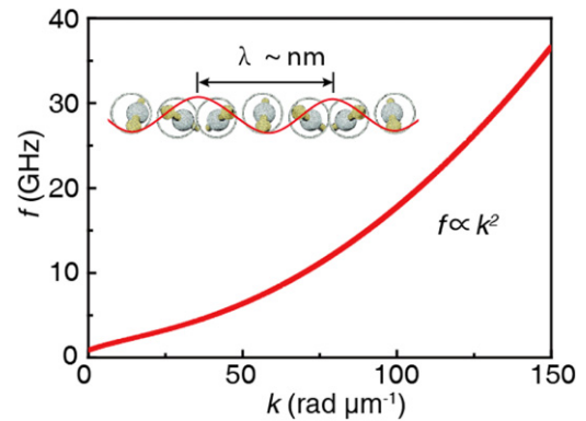
Figure 12. Dispersion for short-wavelength spin waves in YIG (20 nm thickness, saturation magnetization 140 \text{ kA m}^{-1} , exchange constant 3 \times 10^{-16} \text{ m}^2 ) where the propagation direction is perpendicular to the magnetization. At large k (small wavelength \lambda ) the dispersion relation follows a f \propto k^2 behavior dominated by the exchange interaction.
