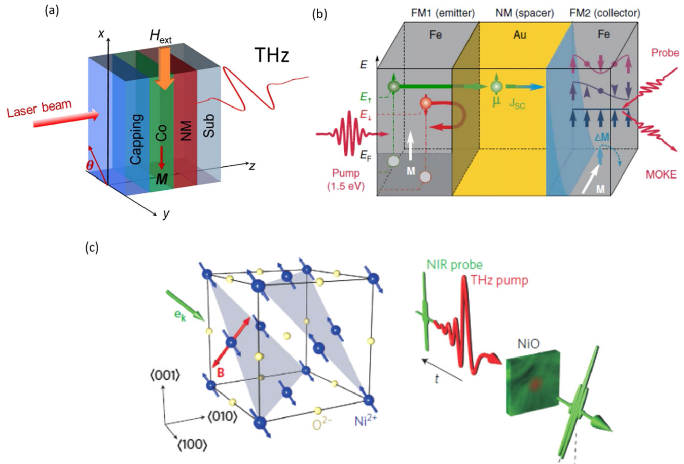
Figure 25. (a) A typical ferromagnet (FM)/non-magnet (NM) sample structure and the THz emission geometry. The femtosecond laser beam is used for pumping the sample. The external magnetic field ( H_{\text{ext}} ) is along the x -axis. In (b) and (c) two strategies are shown to excite spin waves using THz pulses in the THz frequency range. (b) Laser-induced excitation of spin dynamics via spin currents pulses. Due to the spatial confinement of the STT perturbation (blue shaded area), spin waves with a broad spectrum of nonzero wavevectors are excited and can be probed by the MOKE in the collector. The exchange standing spin waves are confined in nanometer thick layer, where the frequency increase as \sim k^2 . Reproduced from [165]. CC BY 4.0. (c) Crystal lattice of NiO with antiferromagnetically ordered spins (blue arrows) in the (111) planes (light blue) and the direction of the THz magnetic field B (double-ended red arrow). An intense free-space THz interacts with the electron spins of a sample to launch a coherent magnon wave. Here the intrinsic modes are in the THz frequency range. A femtosecond near-infrared (NIR) probe pulse (green curves) measures the induced net magnetization by the Faraday effect. Reprinted by permission from Springer Nature Customer Service Centre GmbH: [Springer Nature] [Nature Photonics] [165] (2011).
