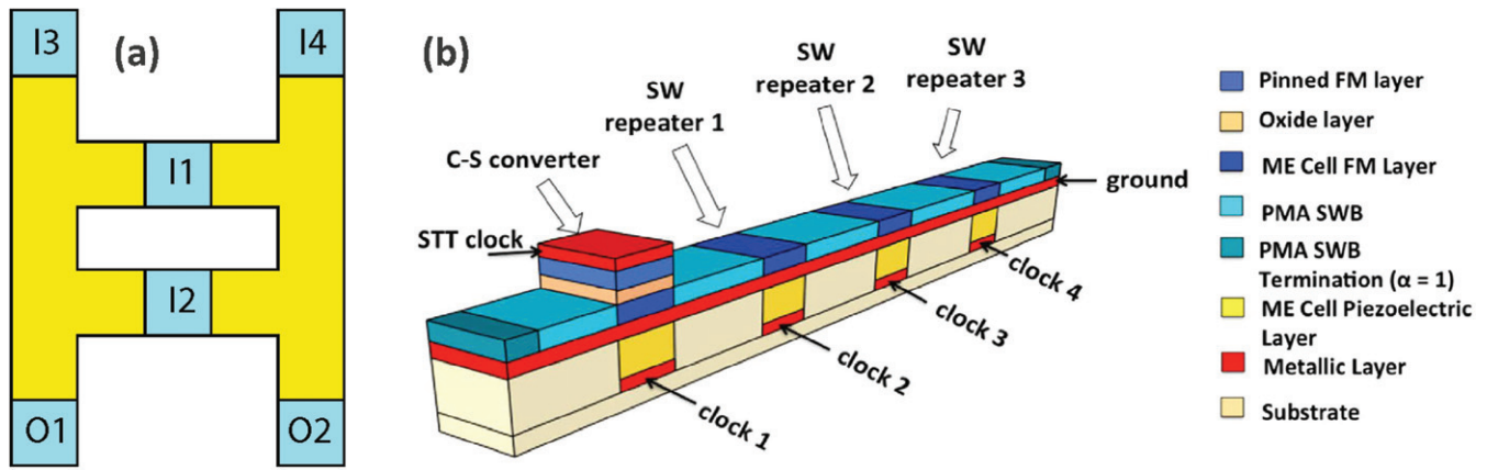
Figure 6. (a) Fan-out enabled spin-wave majority gate with four inputs (I) and two output (O) ports. Reproduced from [48].
