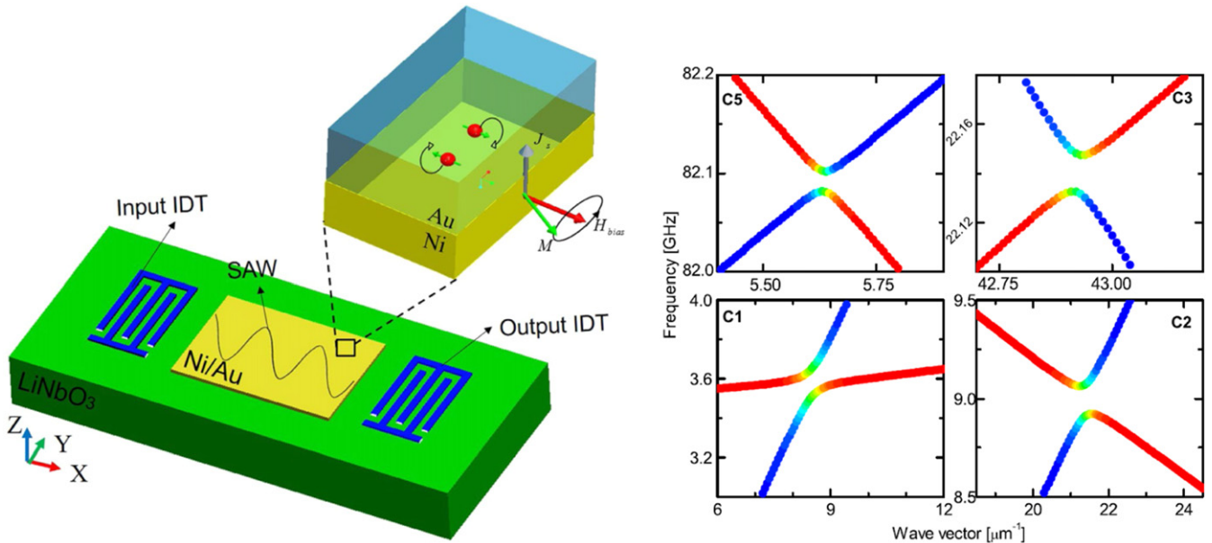
Figure 15. Left panel: SAW driven FMR in magnetostrictive element placed between two interdigital transducers (IDTs) on a single crystal piezoelectric substrate lithium niobate (LiNbO 3 ). Li et al show in reference [100] that the resonant coupling induces SW generation and spin pumping ( J_s in the figure is the spin current induced by magnetization precession). Reprinted from [100], with the permission of AIP Publishing. Right panel: dispersion relation of the NiFe/Co magnonic phononic crystal calculated by Graczyk et al in reference [109]. In the color scale, blue and red correspond to acoustic and spin waves, respectively. Green indicates coupled magnetoelastic waves. Reprinted (figure) with permission from [109], Copyright (2017) by the American Physical Society.
