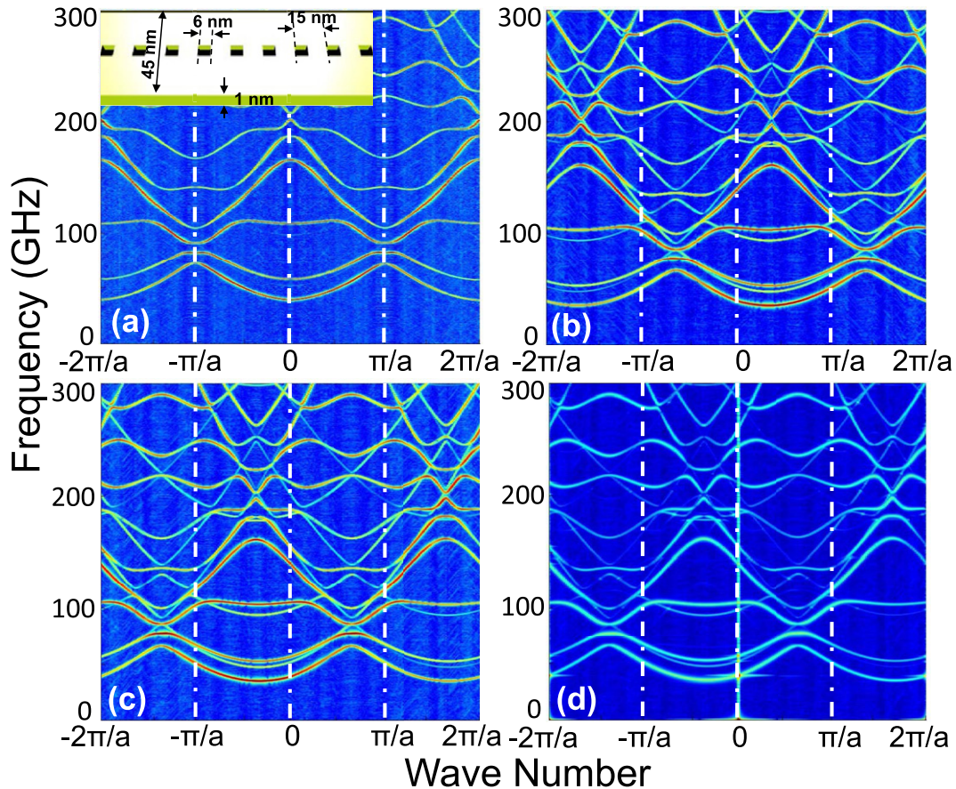
Figure 23. (a) Simulated spin-wave dispersion curves for a one-dimensional \text{Ni}_{80}\text{Fe}_{20} antidot waveguide with 3\ \mu\text{m} length and other dimensions as shown in the schematic at the inset. The spin-wave dispersion is calculated in the DE geometry in presence of a bias magnetic field of 1.01 T. Further application of iDMI strength of (b) D = -2\ \text{mJ m}^{-2} and (c) D = 2\ \text{mJ m}^{-2} have dramatically modified the spin-wave dispersion curves. (d) Application of a current density of 1 \times 10^{11}\ \text{A m}^{-2} on (c) has reduced the spin-wave amplitude significantly. The color map of the spin-wave dispersion is jet, i.e. red corresponds to maximum and blue corresponds to minimum spin-wave amplitude.
