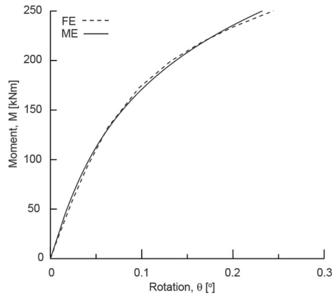
Figure 2. Monotonic load: comparison between finite element and macroelement results
