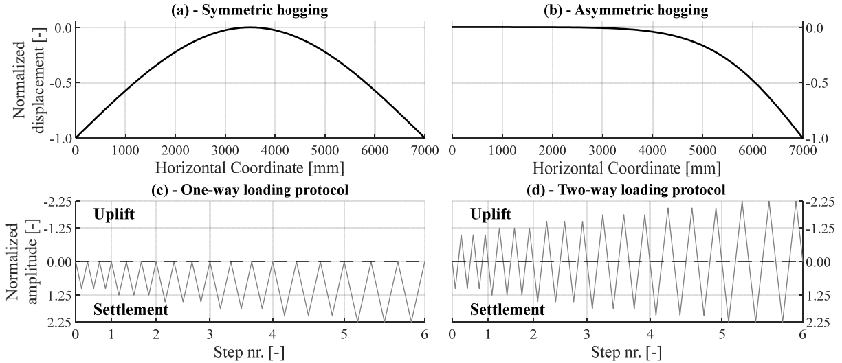
Figure 2: The imposed settlement shapes: (a) symmetric hogging and (b) asymmetric hogging. The adopted loading protocols are (c) one-way and (d) two-way.
