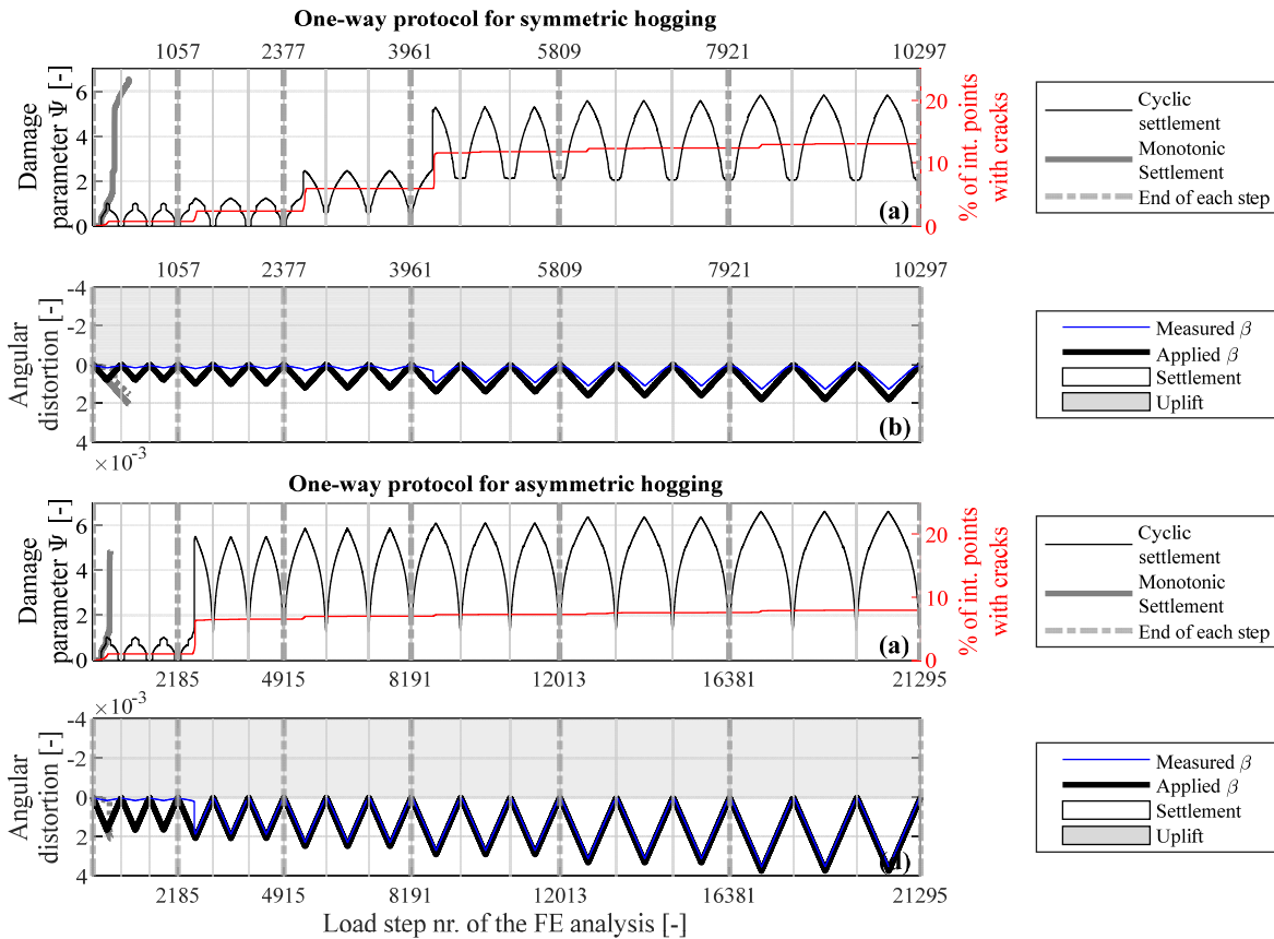
Figure 5: Results for the one-way protocol, load step number against angular distortion \beta and the damage \Psi : (a) and (b) for symmetric, and (c) and (d) for asymmetric hogging.
