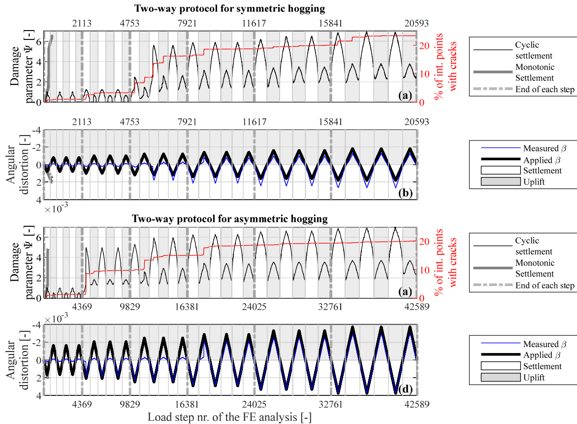
Figure 6: Results for the two-way protocol, load step number against angular distortion \beta and the damage \Psi : (a) and (b) for symmetric, and (c) and (d) for asymmetric hogging.
