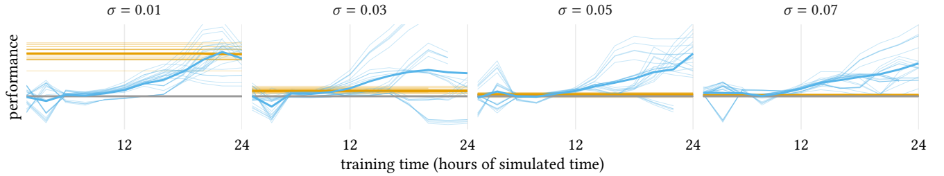
Figure 6: Rewards in the noisy observations benchmark. The gray line (bottom) is the baseline method, the orange horizontal line is FLORIS, and the blue lines show the learning progress of SAC.
