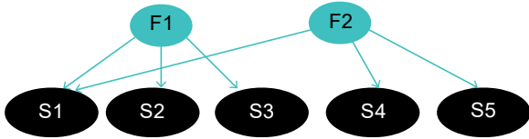
Fig. 4. DBN Structure
