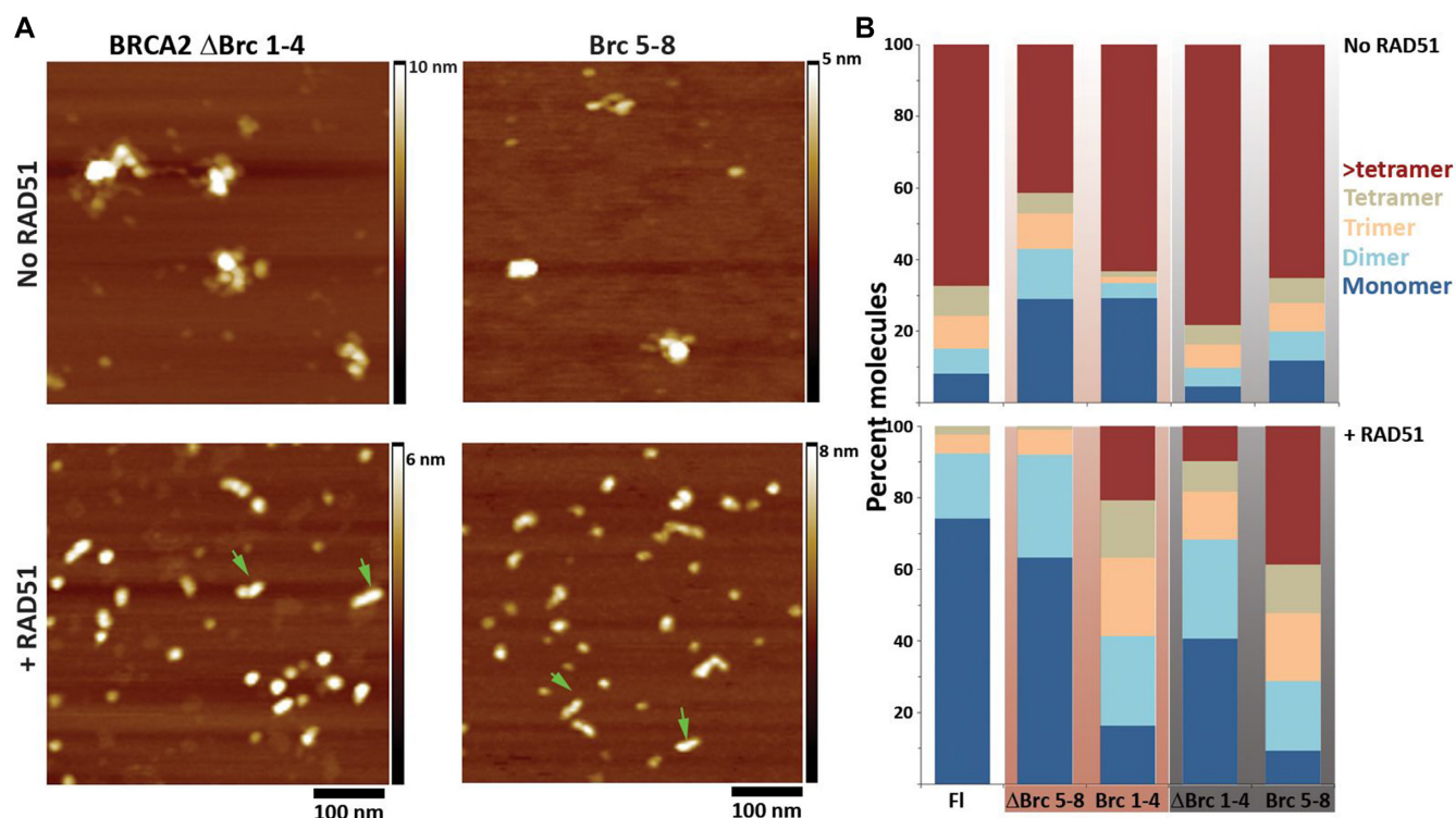
Figure 4. Brc repeats of BRCA2 contribute synergistically to the conformational landscape of the full-length protein. (A) Representative SFM height images of BRCA2 \Delta Brc 1–4 (left panel) and Brc 5–8 (right panel) in the absence and presence of RAD51. Green arrows highlight compact elongated assemblies in the presence of RAD51. The representative images do not necessarily depict the most populous molecular assemblies but are aimed to show, as much as is possible in a single image, the range of architecture of BRCA2 constructs. Note: The Z-scale in the images is different to allow optimal visualization of molecules. (B) Oligomeric distribution of fl, BRCA2 \Delta Brc 5–8, Brc 1–4, BRCA2 \Delta Brc 1–4 and Brc 5–8 in the absence (top panel) and presence (bottom) of RAD51. Brc 1–4 and Brc 5–8 are controls for BRCA2 \Delta Brc 5–8 and BRCA2 \Delta Brc 1–4, respectively. Distinct oligomeric profiles of the two groups, highlighted in red and grey rectangles, on interaction with RAD51 show that Brc 1–4 and Brc 5–8 are biochemically distinct in isolation.
