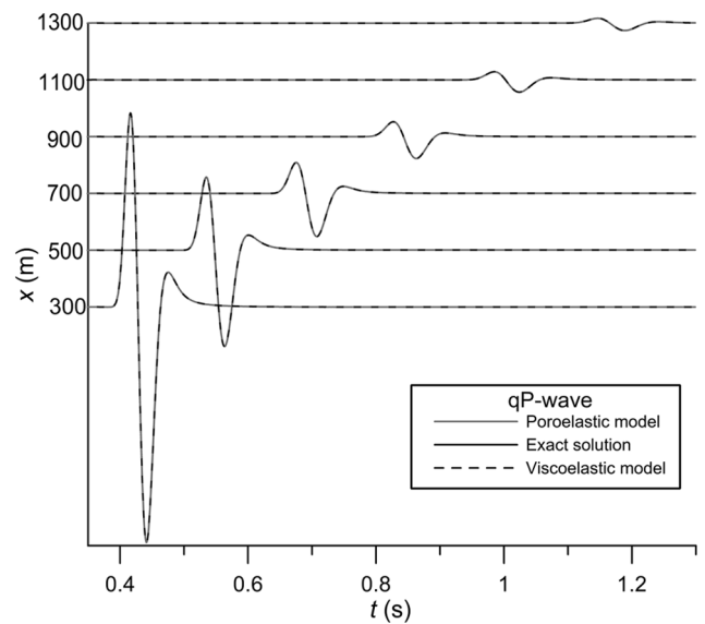
Figure 3. The qP-waveforms at a depth z = 400 m for different x . The medium consists of water- and CO 2 -saturated sandstone layers, l_1 = l_2 = 0.2 m, f_R = 200 Hz. All three lines coincide.
