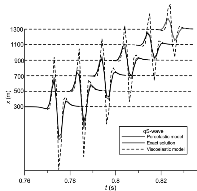
Figure 4. The qS-waveforms at a depth z = 400 m for different x . The medium consists of water- and \text{CO}_2 -saturated sandstone layers, l_1 = l_2 = 0.2 m, f_R = 200 Hz. The actual arrival times are not shown here, the interval between the arrival times t = 0.01 s is chosen for visualization purposes.
