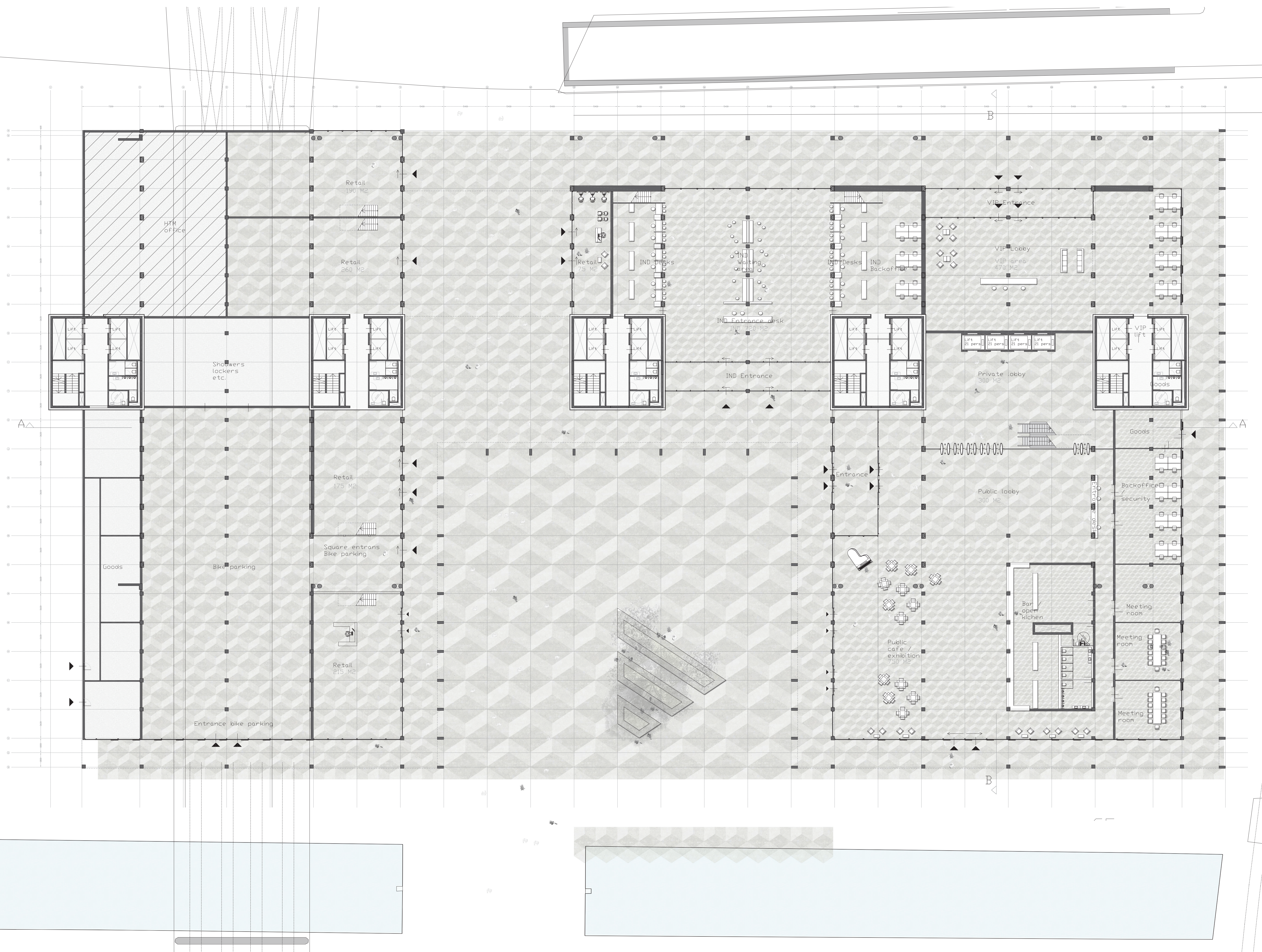
Ground floor. Scale 1:200
