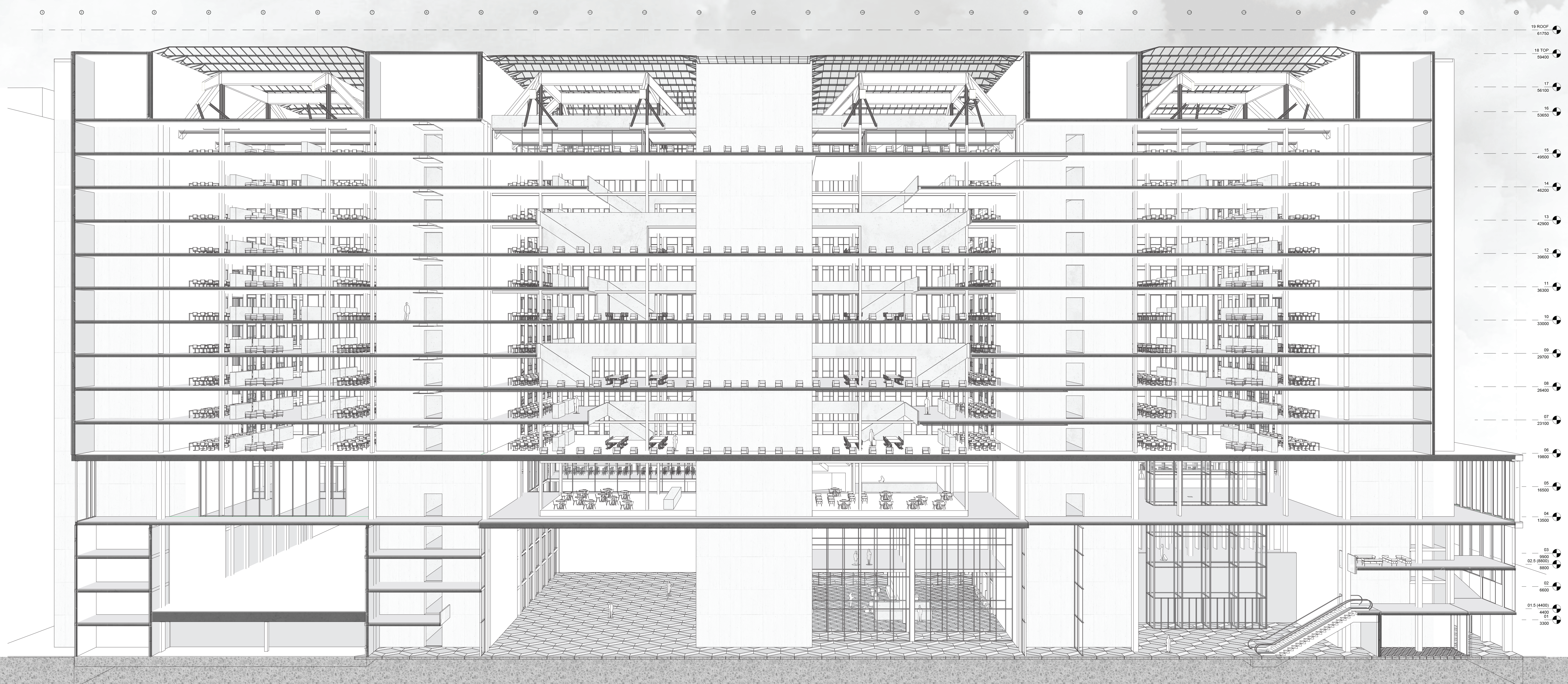
section of perspective A-A' Scale 1:200
