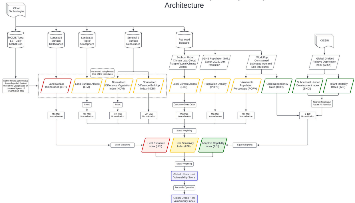
Fig. 1. GUHVI architecture diagram, indicating data sources, normalization, and equal weighting approaches.
