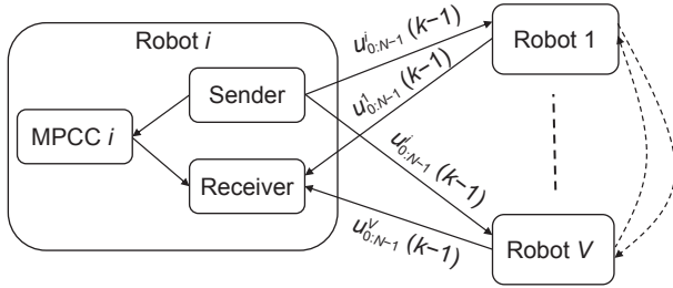
Fig. 4 Multi-robot system architecture.
