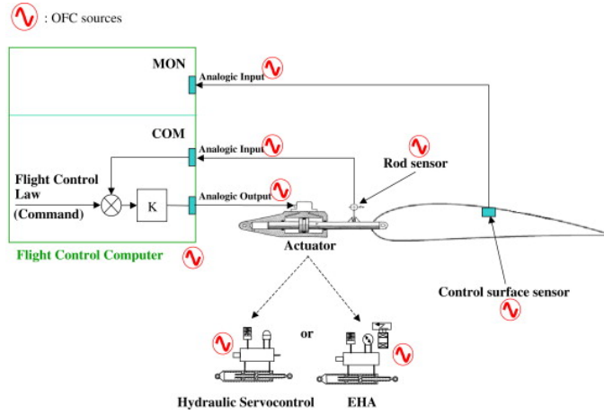
Figure 1.3: Schematic of a servo-control loop with potential sources of an OFC. [13]
