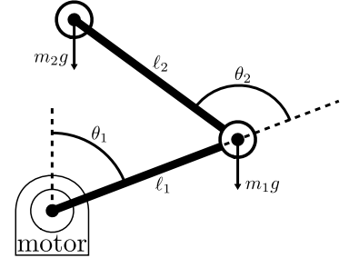
Figure 4.3: Double pendulum as modeled by Equation (4.20).
