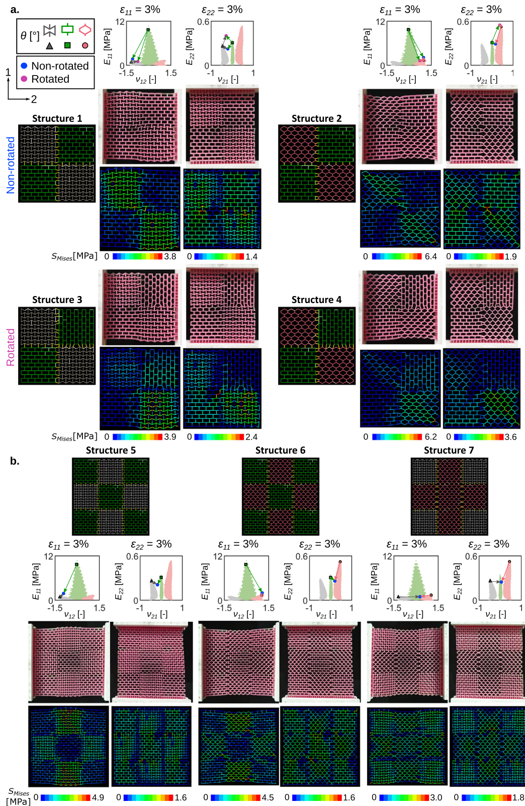
Fig. 3 Different combinations of designs with extreme mechanical properties. These designs are selected from each group of the unit cells (i.e., a re-entrant structure with a highly negative Poisson's ratio, a honeycomb structure with a highly positive Poisson's ratio, and an orthogonal structure with a high value of the elastic modulus). a The mechanical properties of two four-tile structures with non-rotated and rotated tiles and the distribution of the von Mises stresses in these lattice structures. These multi-material 3D printed specimens were mechanically tested in both the 1- and 2-directions under 3% tensile strain and the experimental results were compared with the FE simulation results (Table 1). b The mechanical properties of nine-tile combinations and the von Mises stress distribution in these combinations. These multi-material 3D printed specimens were mechanically tested in both the 1- and 2-directions under 3% tensile strain, and the experimental results were compared with the FE simulation results (Table 1).
