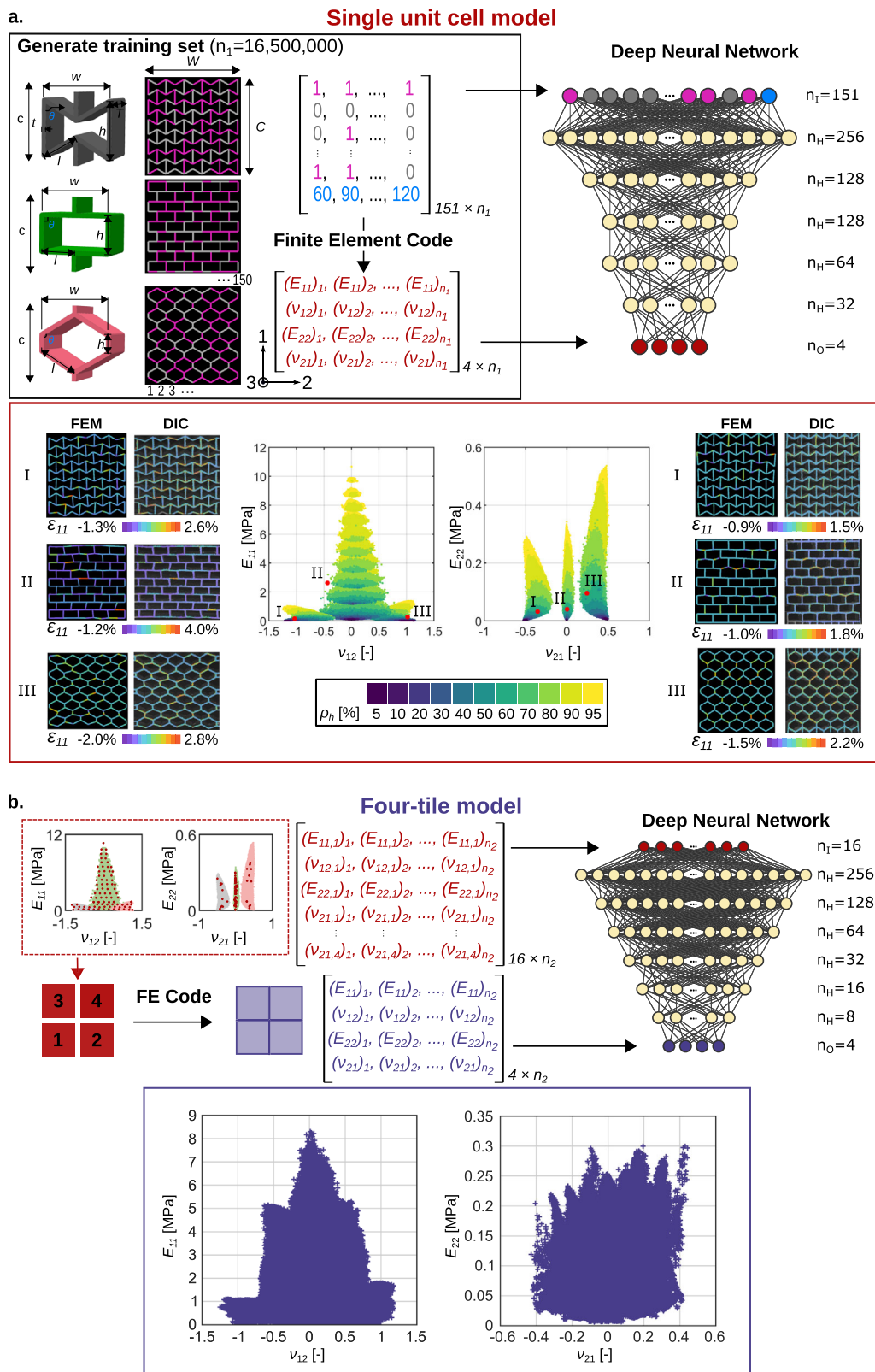
Fig. 1 The structures of the optimized deep learning models as well as relevant training procedures and the range of attainable mechanical properties.
