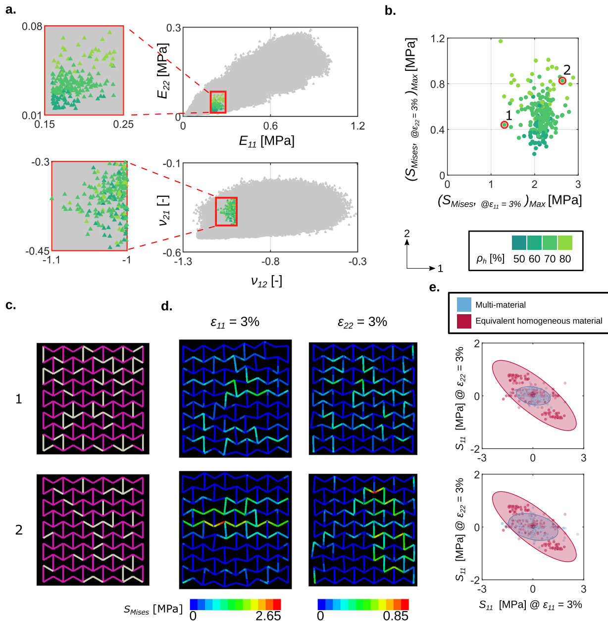
Fig. 4 Stress distribution within the lattice structure. a The selection of a certain range of the elastic properties achieved for the unit cells with a cell angle of 60°. In total, the elastic properties of 207 designs with various \rho_h values (i.e., 50%, 60%, 70% and 80%) fall within these selected ranges. b The maximum values of the von Mises stress in the structural elements of the corresponding lattice structures when these structures were subjected to two boundary conditions (i.e., \epsilon_{11} = 3\% or \epsilon_{22} = 3\% ). Two designs were selected, including one with the minimum (node 1) and one (node 2) with the maximum Euclidean distance from the origin ( b , c ). The distribution of the von Mises stresses in the selected designs and their deformations under two boundary conditions (i.e., \epsilon_{11} = 3\% or \epsilon_{22} = 3\% ) are presented in ( d ). The axial stresses ( S_{11} ) in the struts of each design under two boundary conditions (i.e., \epsilon_{11} = 3\% or \epsilon_{22} = 3\% ) are calculated and are compared with the axial stresses of the corresponding struts when the lattice structure is composed of an equivalent homogeneous material ( e ).
