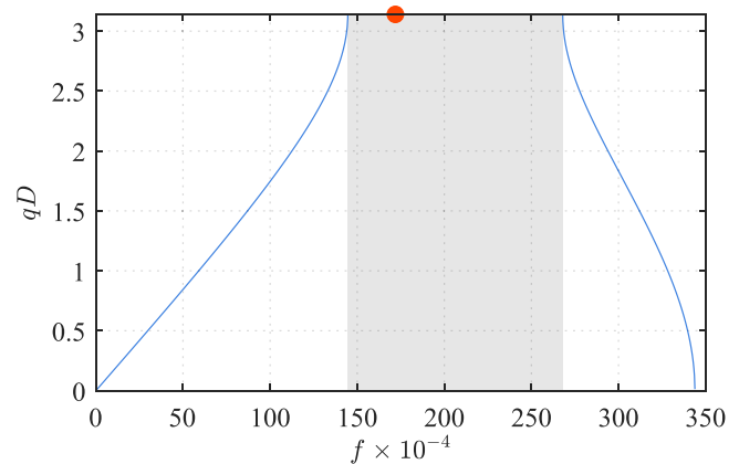
FIG. 3. Analytical dispersion curve of the three layer unit cell design. Shaded region: stop band; red mark: resonance mode eigenfrequency (0.0172, 300.71 Hz).
