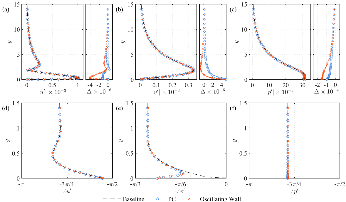
FIG. 7. Comparison of shape functions (a)–(c) and phase angles (d)–(f) of u' , v' , and p' between baseline, oscillating wall, and PC cases pertaining to out-of-phase conditions (0.0174, 304 Hz) at the PC location. The insets in (a)–(c) correspond to the difference with respect to the baseline case (e.g., \Delta = |u'| - |u'|_{\text{base}} ).
