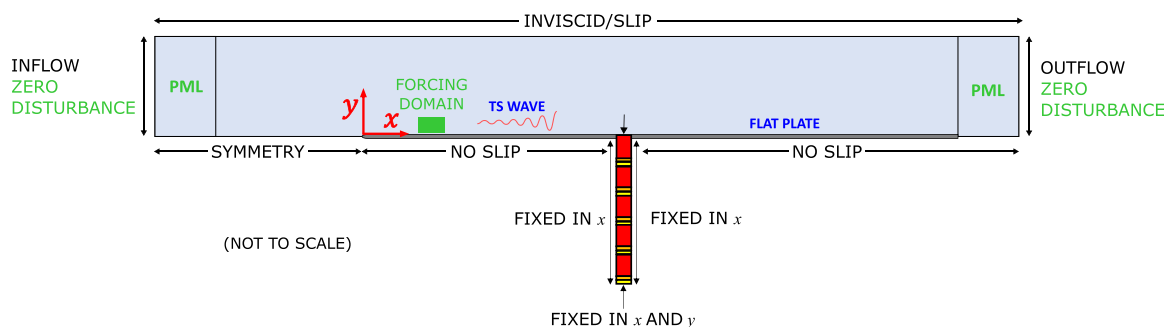
FIG. 1. An illustration of the geometry and simulation boundary conditions. Black and green font descriptors pertain to the boundary conditions for the steady state and frequency domain simulations, respectively. PML: perfectly matched layer.
