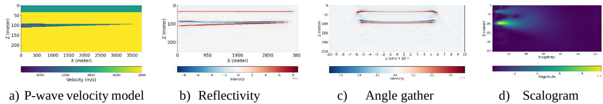
Figure 1 The sample geological model, its corresponding reflectivity, the angle gather at x=1900 m, and the zero-angle scalogram.
