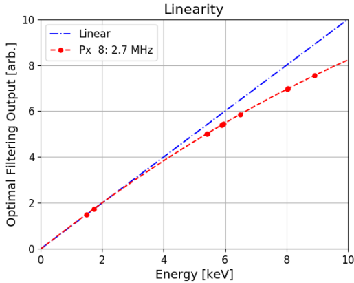
Fig. 8. Detector linearity in the range from 1.5 to 9 keV. The optimal filtering output is shown as a function of the detected line energies (red points). The dashed blue line is the linear trend calibrated on the low energy lines.
