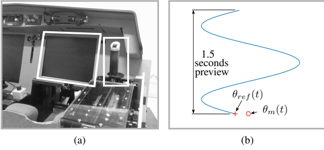
Fig. 3. (a): The apparatus used in the JND experiment. The side-stick manipulator and the LCD screen are marked by white rectangles. The LCD screen only displays the visual presentation of the tracking task. (b): The tracking task shown on the LCD screen. To reduce the manipulator deflection tracking error exemplified in this figure, the subject has to push the manipulator towards the left.
