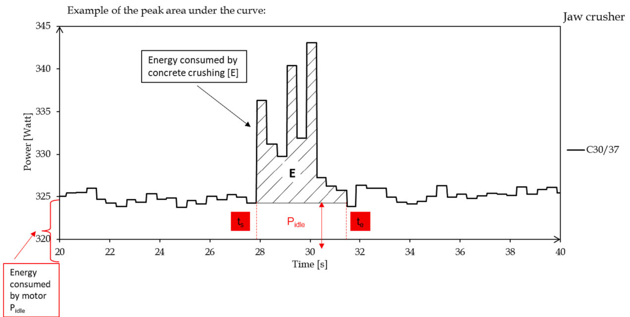
Fig. 6. Determination of cumulative energy used for concrete crushing.
