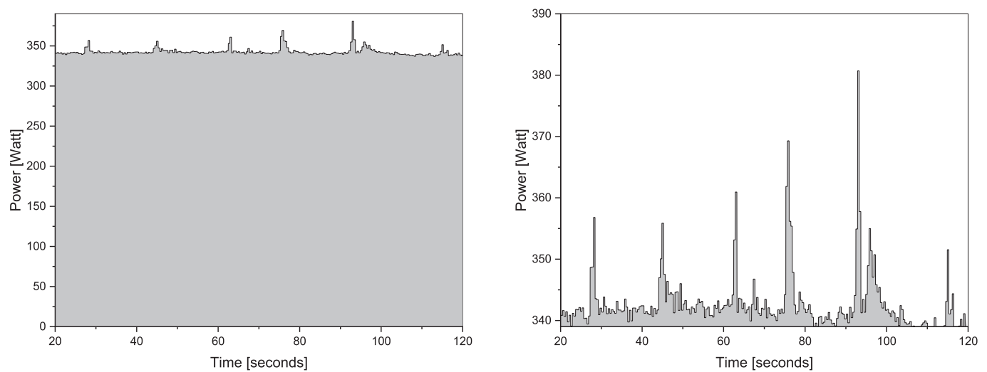
Fig. 10. (In)efficiency of the motor. The motor power is much higher than the power needed for concrete crushing.
