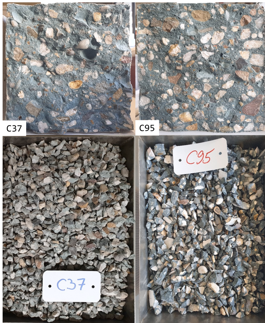
Fig. 9. Fracture in C30/37 and C80/95 specimens after tensile splitting strength test, and shape of RCA sieved for Los Angeles test with a particle size between 10 and 14 mm obtained after dried sieving.
