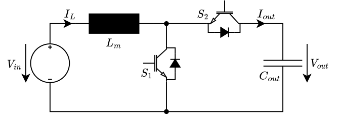
Fig. 3. Equivalent circuit of ideal half-bridge DCDC converter
