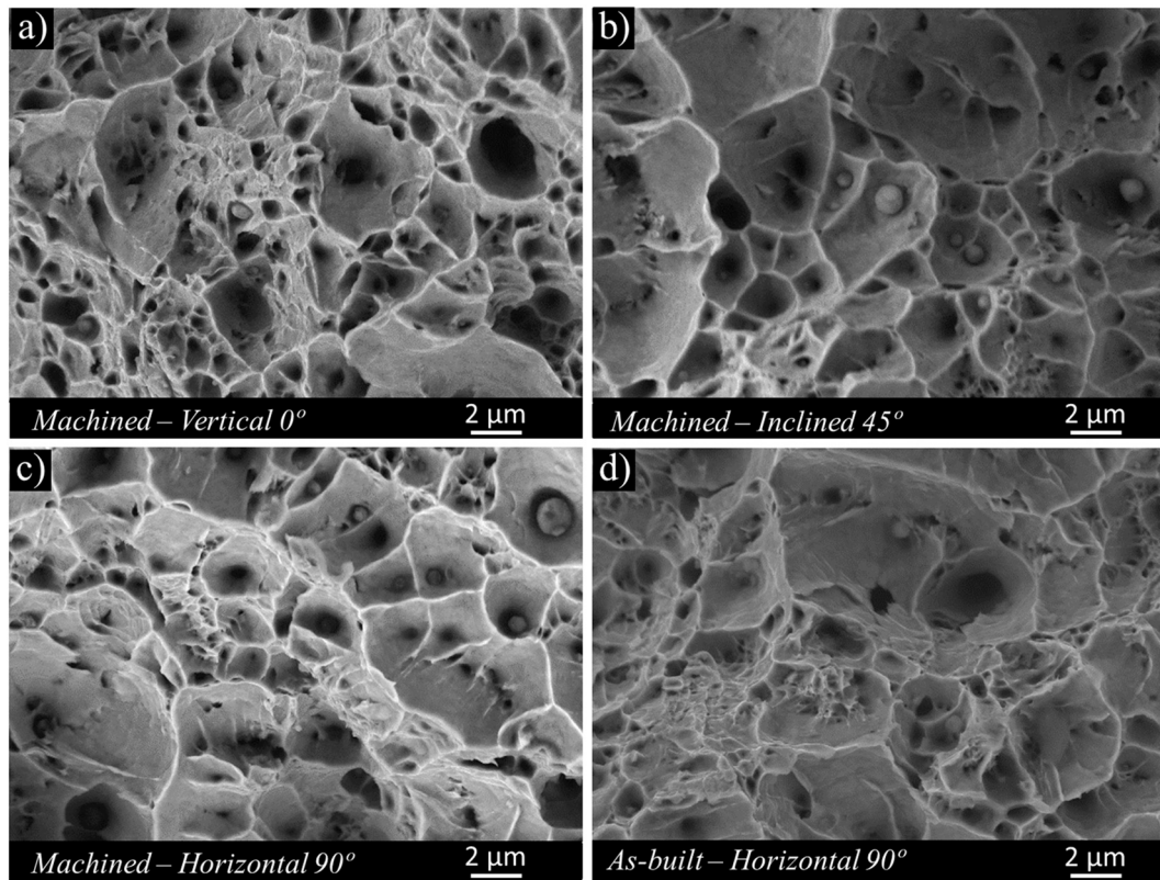
Fig. 12. High-magnification micrographs of the fibrous region (central region of the fracture surfaces): (a) vertical, as-machined condition; (b) inclined, as-machined condition; (c) horizontal, as-machined condition; (d) horizontal, as-built condition.
