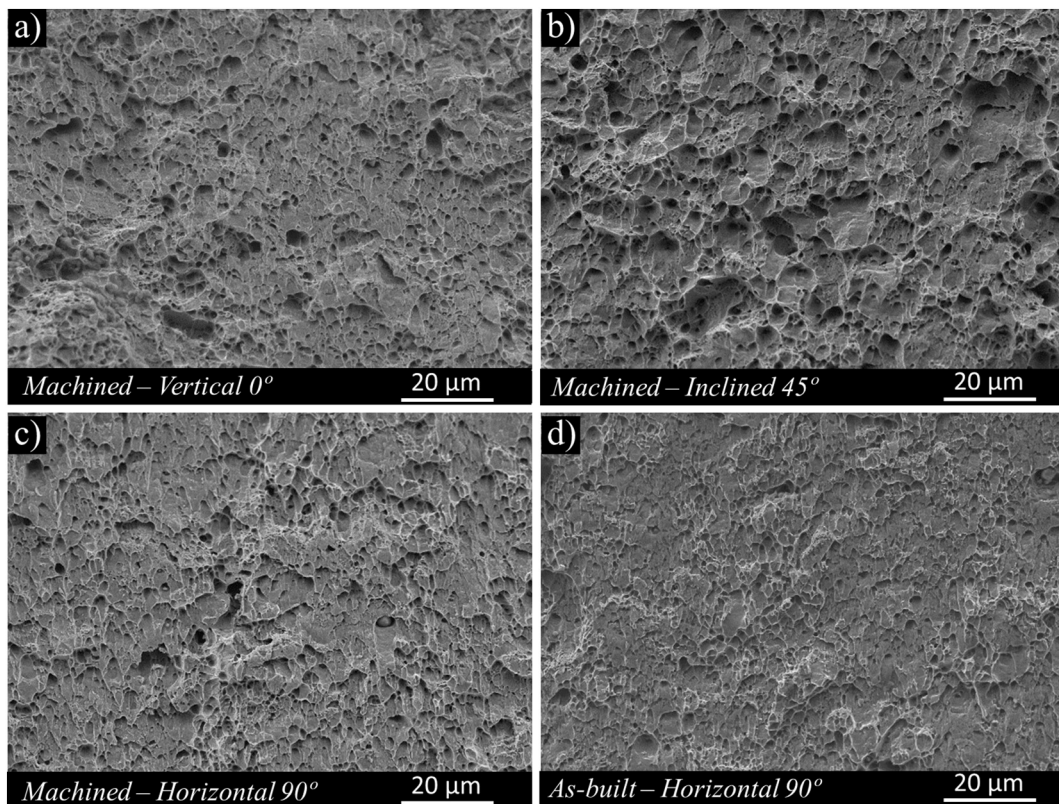
Fig. 11. Micrographs of the smoother region surrounding the fibrous region: (a) vertical, machined condition; (b) inclined, machined condition; (c) horizontal, machined condition; (d) horizontal, as-built condition.
