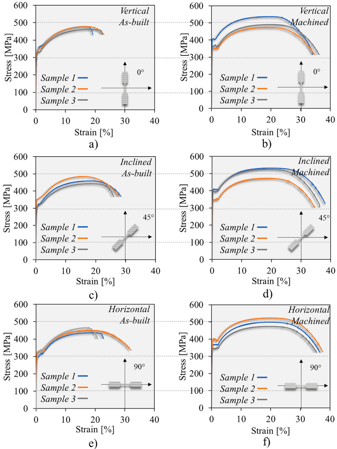
Fig. 4. Stress-strain curves for the (a, c and e) as-built and (b, d and f) machined coupons with various orientations: 0° (vertical), 45° (inclined) and 90° (horizontal), relative to the print layer direction.
