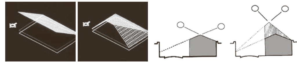
11 Solar plane and solar envelope. [Karen Kense] 12 Shadow fences. [Ralph Knowles]
