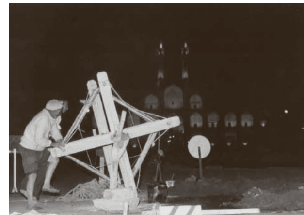
16 Qanat-builders at work today. [Masoud Abtahi, Courtesy of Bayana Bogasari]
