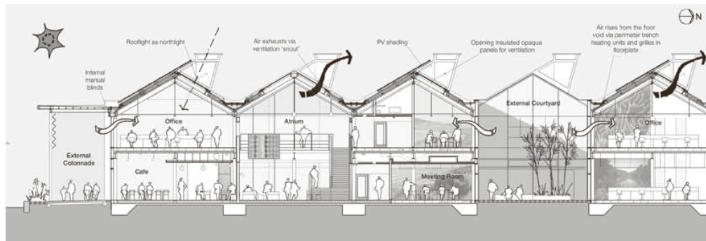
6 Building Section, Heelis Building, National Trust Headquarters, Swindon, UK, [Freidlen Clegg & Bradley Studios]
