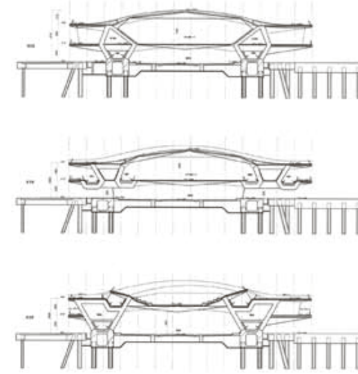
2 Transverse Sections, Yokohama International Port Terminal, Yokohama, Japan, Foreign Office Architects, 2002. [Foreign Office Architects]
