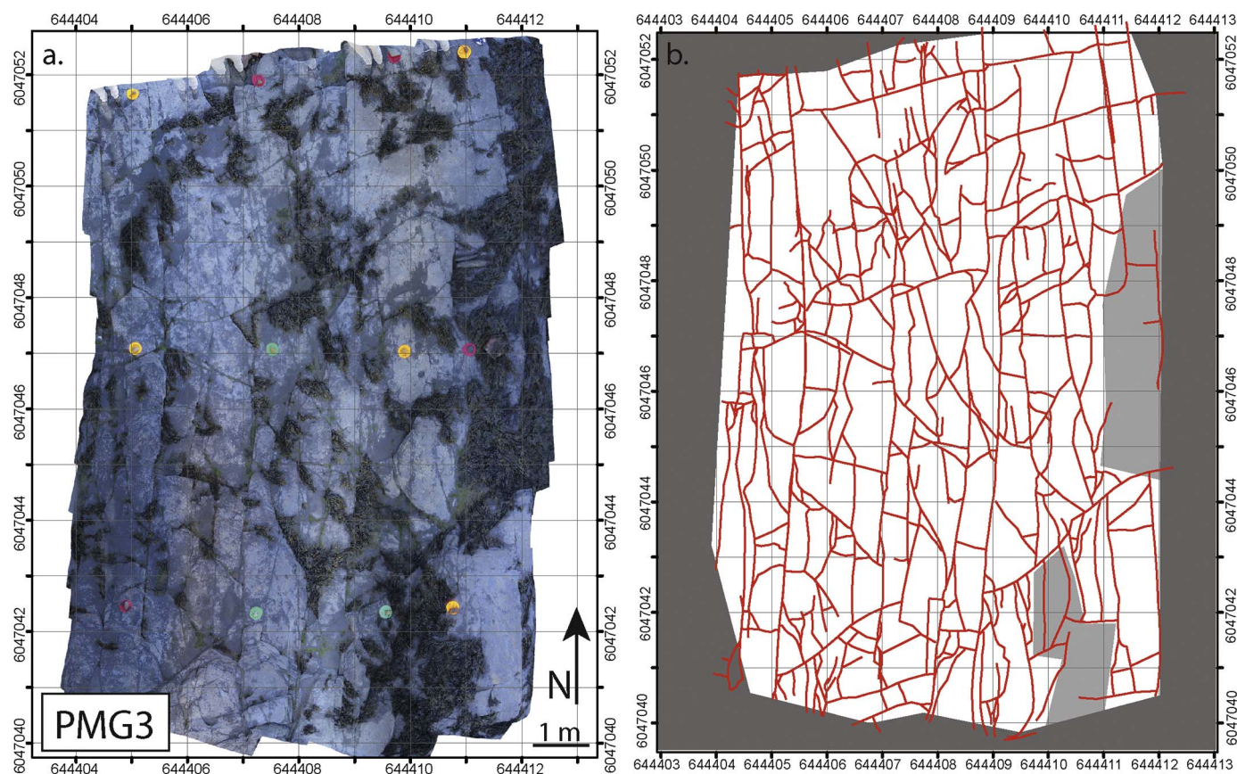
Fig. 5. a. Captured photo mosaic of one of the imaged domains. Colored circles are the Frisbees used as ground-control-points for which UTM coordinates were measured with GPS. b. The fracture network as captured from the imaged domain with some areas badly exposed due to boulders, gravel and/or seaweed on the surface of the pavement. (For interpretation of the references to colour in this figure legend, the reader is referred to the web version of this article.)
