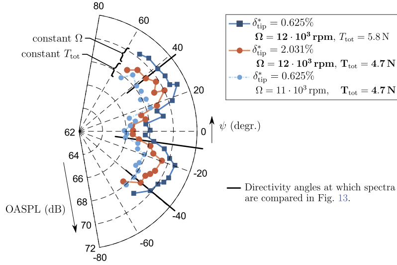
Fig. 12. Overall sound pressure level (OASPL) at a distance of R_a = 10D_d , plotted against the directivity angle, \psi . Directivity patterns are compared for two tip-gap ratios \delta_{tip}^* , at the same rotational speed ( \Omega = 12000 rpm), as well as at the same level of thrust ( T_{tot} = 4.7 N). Recall that the three corresponding operating conditions were illustrated in Fig. 11.
