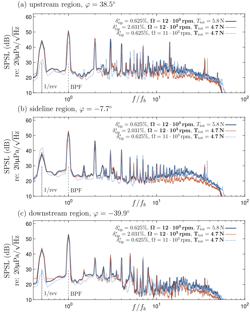
Fig. 13. Acoustic spectra in the (a) upstream, (b) sideline, and (c) downstream regions of the acoustic field; directivity angles are indicated above each set of spectra. Each set of spectra compares two tip-gap ratios \delta_{tip}^* , at the same rotational speed ( \Omega = 12000 rpm), as well as at the same level of total thrust ( T_{tot} = 4.7 N). Recall that the three corresponding operating conditions were illustrated in Fig. 11.
