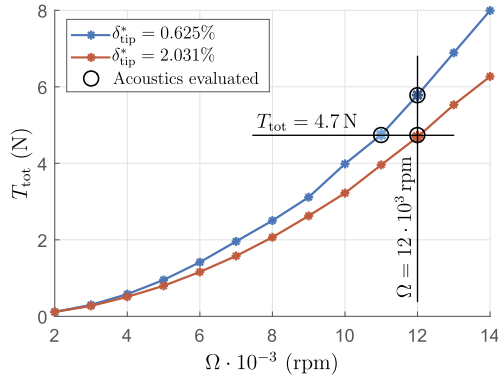
Fig. 11. Illustration of the three operating conditions for the acoustic measurements (open circles), covering a constant total thrust setting T_{tot} , and a constant rotational speed setting \Omega , for the two different tip-gap ratios \delta_{tip}^* .
