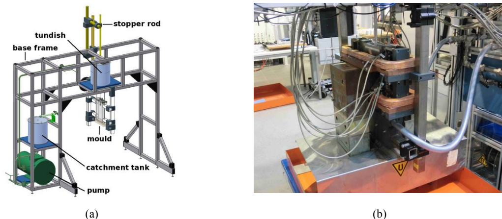
Fig 1.: Schematic (a) and photo (b) of the Mini-LIMMCAST facility
