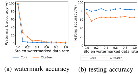
Figure 8: Watermarking performance for different stolen watermarked data rates on node classification (GraphSAGE).
