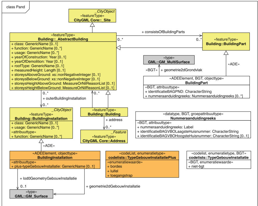
Fig. 11.5 The UML diagram of IMGeo ADE for the CityGML class Building ( Pand in Dutch). The yellow parts are from the CityGML standard; the rest is additional information in the application domain extension. (© Geonovum, reprinted with permission)
