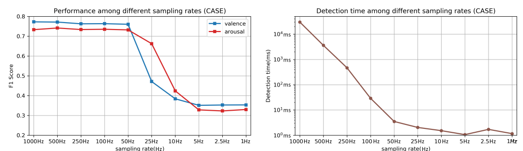
Figure 8. Comparison of the performance among different sampling rates: W-F1 of binary classification (LOSOCV, left) and detection time (right).
