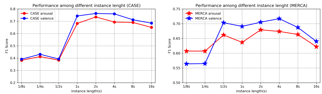
Figure 7. Comparison of the performance among different instance lengths: W-F1 of binary classification (LOSOVC).
