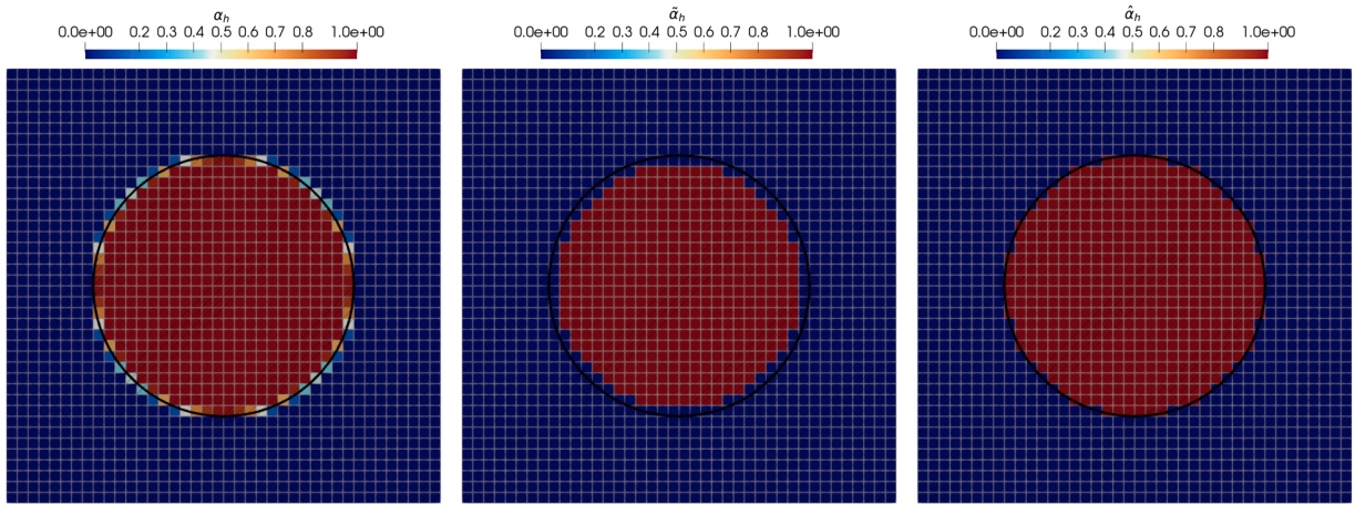
Fig. 4. Volume fraction weights \alpha_h (left), \tilde{\alpha}_h (center) and \hat{\alpha}_h (right).
