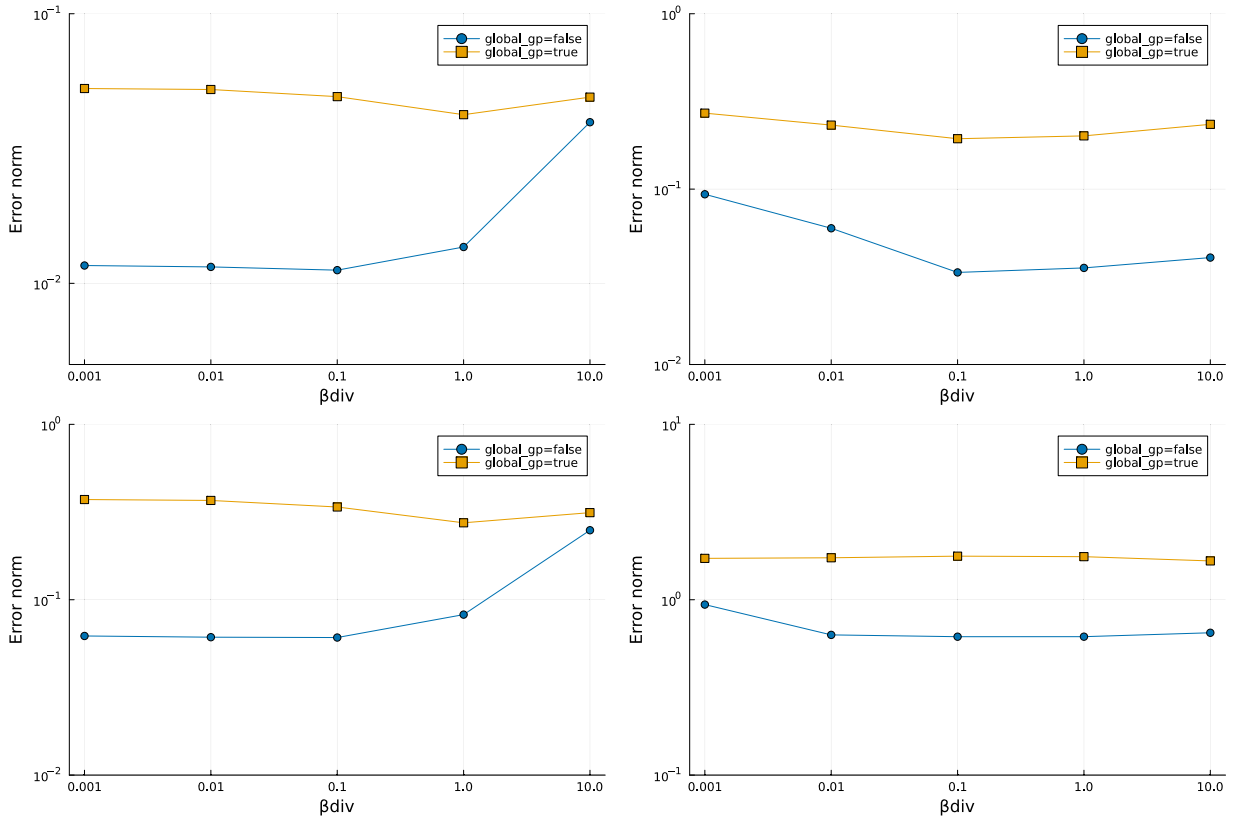
Fig. 24. Sensitivity with respect to the grad-div constant \beta_{div} with and without global ghost penalty. L^2 -norm (top) and L^\infty -norm (bottom) in time of the velocity (left) and pressure (right) L^2 error norm.
