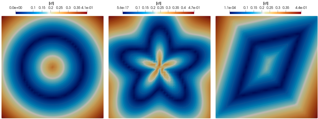
Fig. 3. Distance function magnitude for the circle (left), flower-shape (center) and parallelogram (right).
