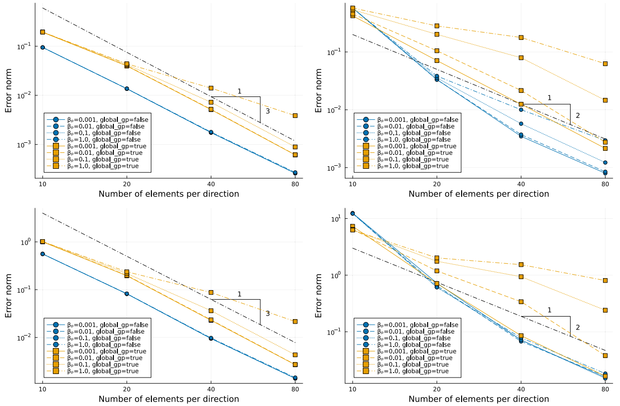
Fig. 23. Sensitivity with respect to the ghost-penalty constant \beta_2^p . L^2 -norm (top) and L^\infty -norm (bottom) in time of the velocity (left) and pressure (right) L^2 error norms.
