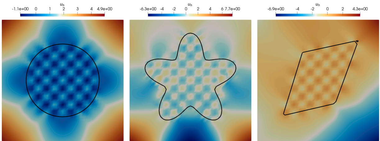
Fig. 5. Computed solution using the WSBM equivalent in a 40 by 40 background grid. Circle level set function (left), flower-shape level set function (center) and parallelogram level set function (right).
