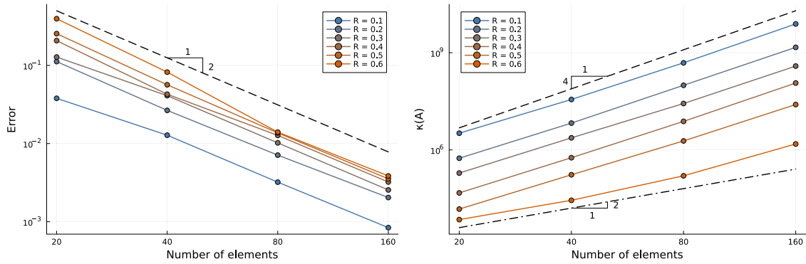
Fig. 9. L^2 -norm of the solution error and condition number of the resulting matrix for varying radius of the circle.
