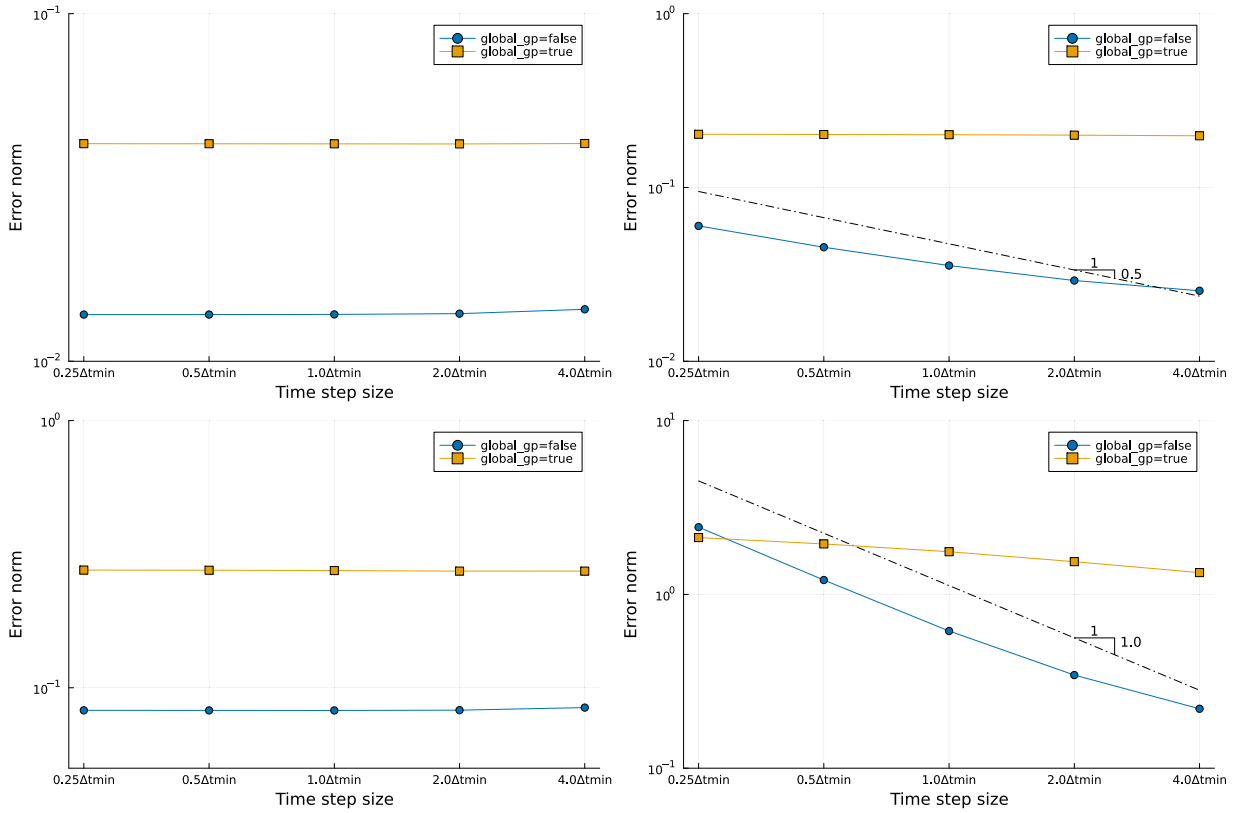
Fig. 22. Sensitivity with respect to the time step size \Delta t with and without global ghost penalty. L^2 -norm (top) and L^\infty -norm (bottom) in time of the velocity (left) and pressure (right) L^2 error norms.
