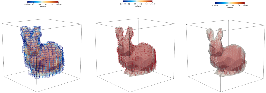
Fig. 13. Geometrical representation of the Low Poly Stanford Bunny in 30 \times 30 \times 30 background grid. The weights are only depicted in active elements ( \alpha_h > 0 ). WSBM (left), O-SBM (center) and SBM (right).
