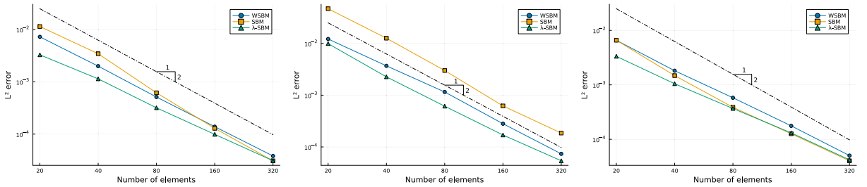
Fig. 17. L^2 -norm of error convergence: circle shape (left), flower shape (center) and quadrilateral (right).
