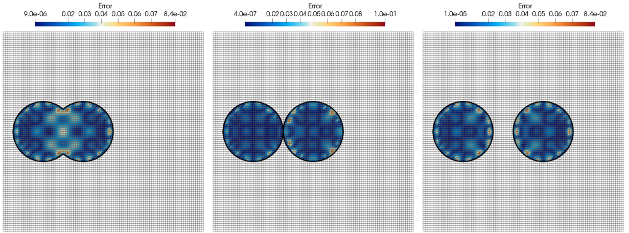
Fig. 12. Solution error at different circles position: d = -0.1 (left), d = 0.0 (center) and d = 0.1 (right). The error is depicted only in the interior of the physical domain ( \Omega ).
