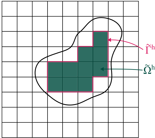
(a) Surrogate domain \tilde{\Omega}^h and surrogate boundary \tilde{\Gamma}^h used in the SBM formulation.
