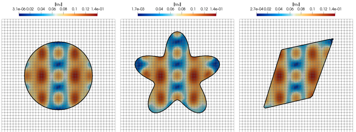
Fig. 15. Computed displacement absolute value using the optimal SBM equivalent in a 40 \times 40 background grid. Circle level set function (left), flower-shape level set function (center) and parallelogram level set function (right). The solution is depicted only in the interior of the physical domain ( \Omega ).
