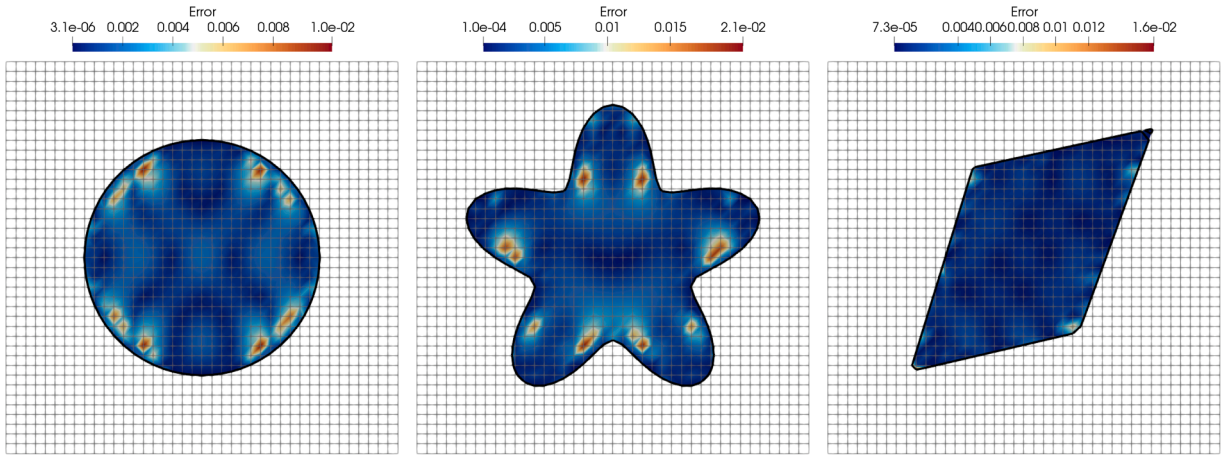
Fig. 16. Absolute value of the displacement error of for the solution computed using the optimal SBM equivalent in a 40 by 40 background grid. Error only depicted in active elements ( \alpha_h > 0 ). Circle level set function (left), flower-shape level set function (center) and parallelogram level set function (right). The error is depicted only in the interior of the physical domain ( \Omega ).
