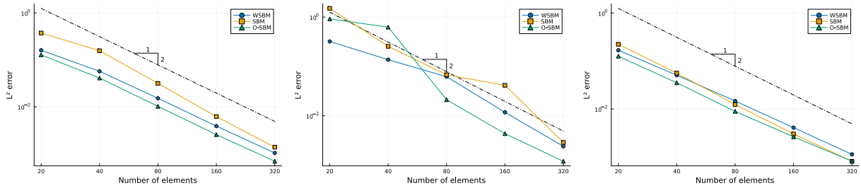
Fig. 7. Convergence of the L^2 -norm using the different weight definitions for the circle level set function (left), the flower-shape level set function (center) and the parallelogram level set function (right).
