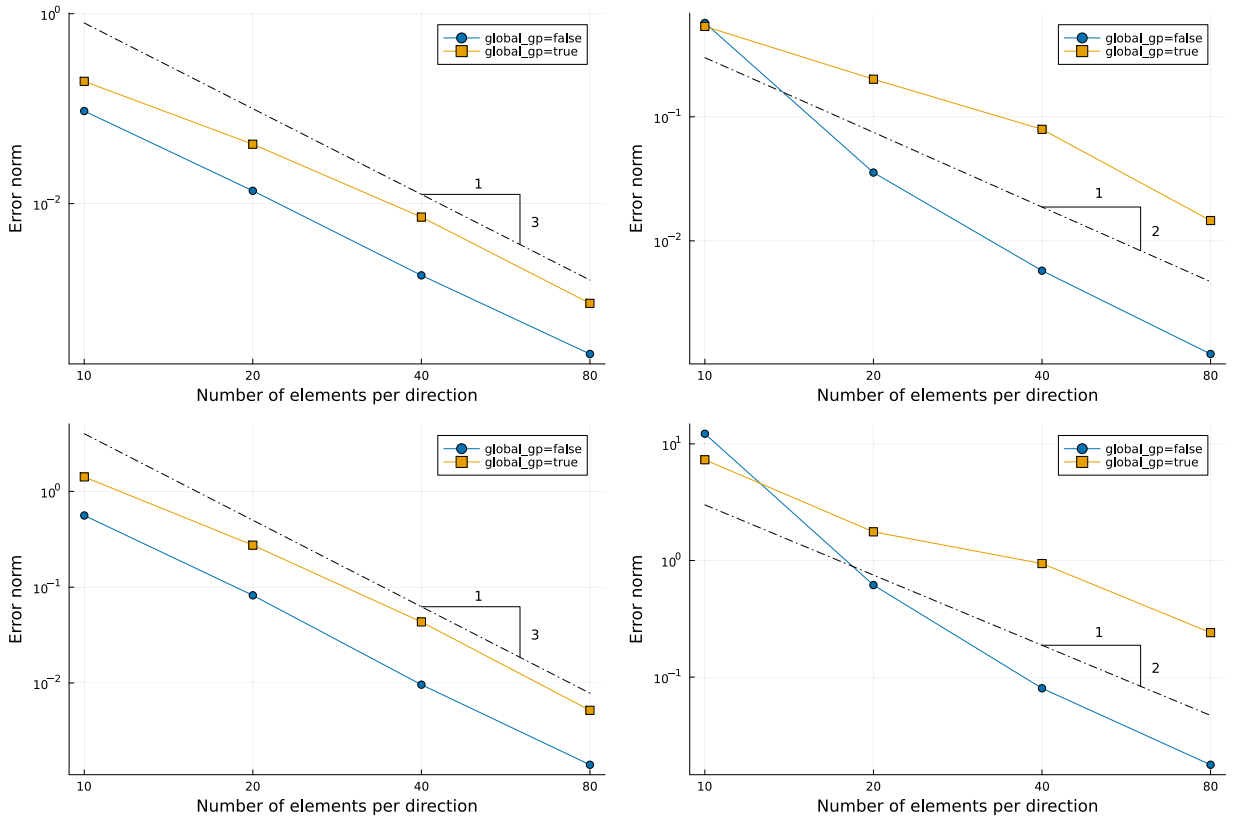
Fig. 21. Convergence in space of the manufactured solution with and without global ghost penalty. L^2 -norm (top) and L^\infty -norm (bottom) in time of the velocity (left) and pressure (right) L^2 error norm.
