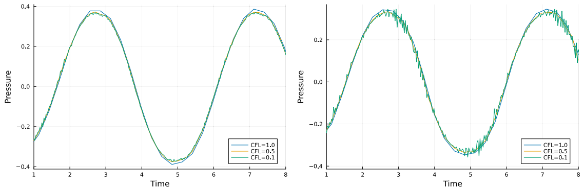
Fig. 28. Pressure value at point [-3.0, 0.0] for the case global\_gp = true (left) and global\_gp = false (right) using different time step sizes equivalent to CFL = \{1.0, 0.5, 0.1\} .
