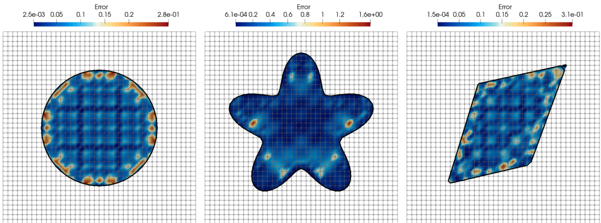
Fig. 6. Absolute value of the error of for the solution computed using the WSBM equivalent in a 40 by 40 background grid. The error is depicted only in the interior of the physical domain ( \Omega ). Circle level set function (left), flower-shape level set function (center) and parallelogram level set function (right).
