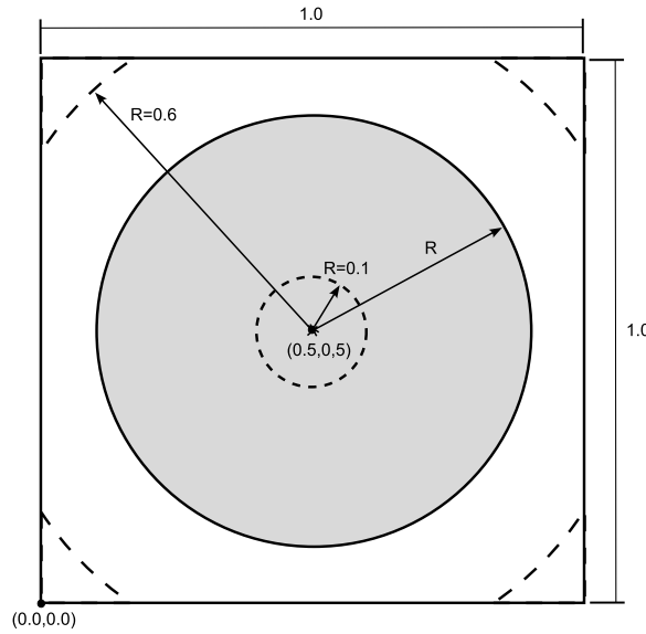
Fig. 8. Sketch of the geometry used in the condition number analysis.
