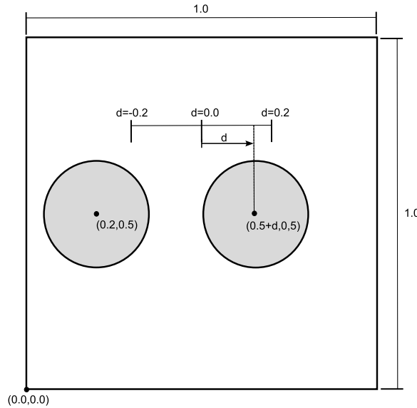
Fig. 10. Sketch of the parametric geometry problem.
