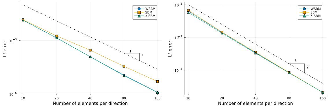
Fig. 20. L^2 -norm of the velocity (left) and pressure (right) error convergence.
