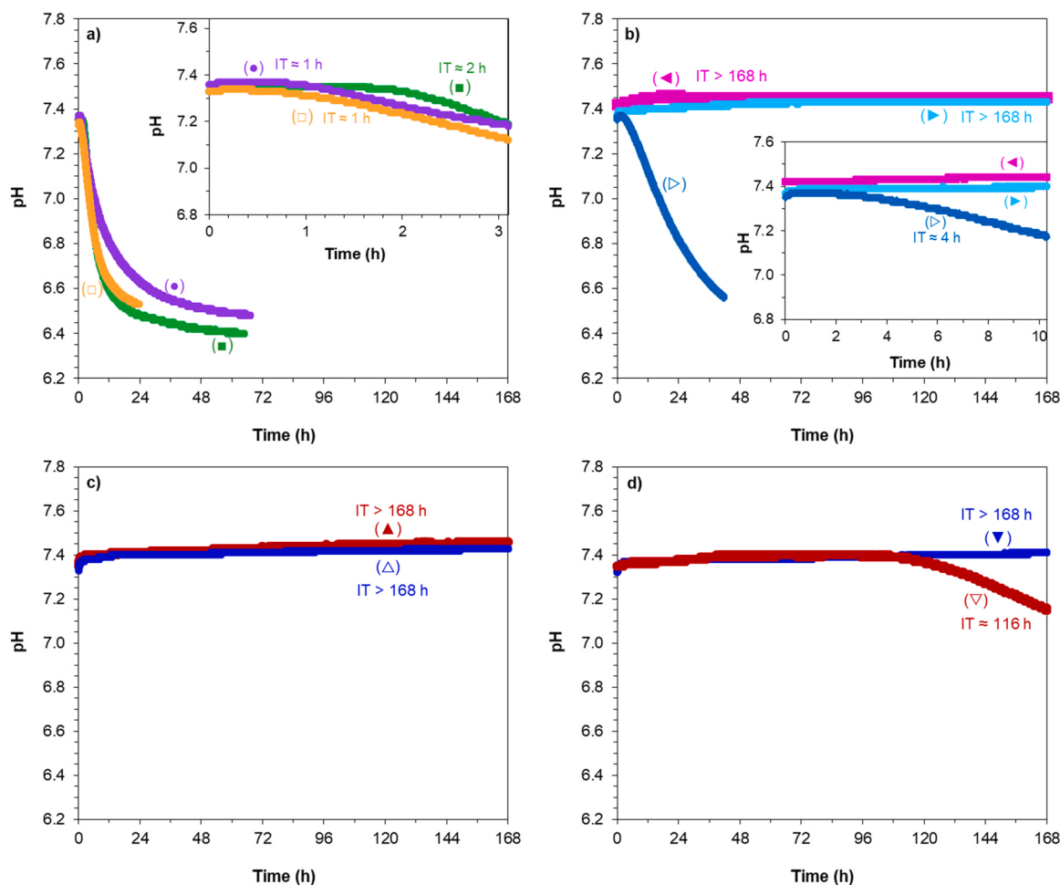
Fig. 7. (a) IT of artificial concentrate of 80% recovery (◐) in the absence of foreign substances, (●) with 217 mg/L sulphate, and (■) with 87 mg/L magnesium, (b) IT of the artificial concentrate of 80% recovery (◑) with 10 mg/L phosphate, (◒) with 5 mg/L phosphate, and (◓) with 2.5 mg/L phosphate, (c) IT of the artificial concentrate of 80% recovery (▲) with 10 mg/L of IHSS FA, and (△) with 5 mg/L of IHSS FA, and (d) IT of the artificial concentrate of 80% (▼) with 10 mg/L of IHSS HA and (▽) with 5 mg/L of IHSS HA.
