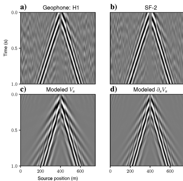
Figure 8. The CRG at 400 m: (a) recorded geophone H_1 , (b) recorded SF-2, (c) modeled V_x , and (d) modeled \partial_x V_x .
