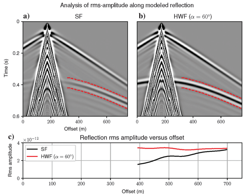
Figure 15. Modeled reflection responses and their rms amplitudes: (a) shots for SF, (b) HWF with wrapping angle of 60^\circ , and (c) the dashed red lines highlight analysis windows of 40 ms to calculate rms amplitudes as a function of offset for the reflection.
