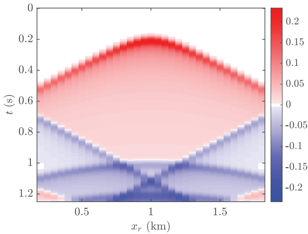
FIGURE 4 Seismogram as function of the horizontal receiver position x_r and time t .
