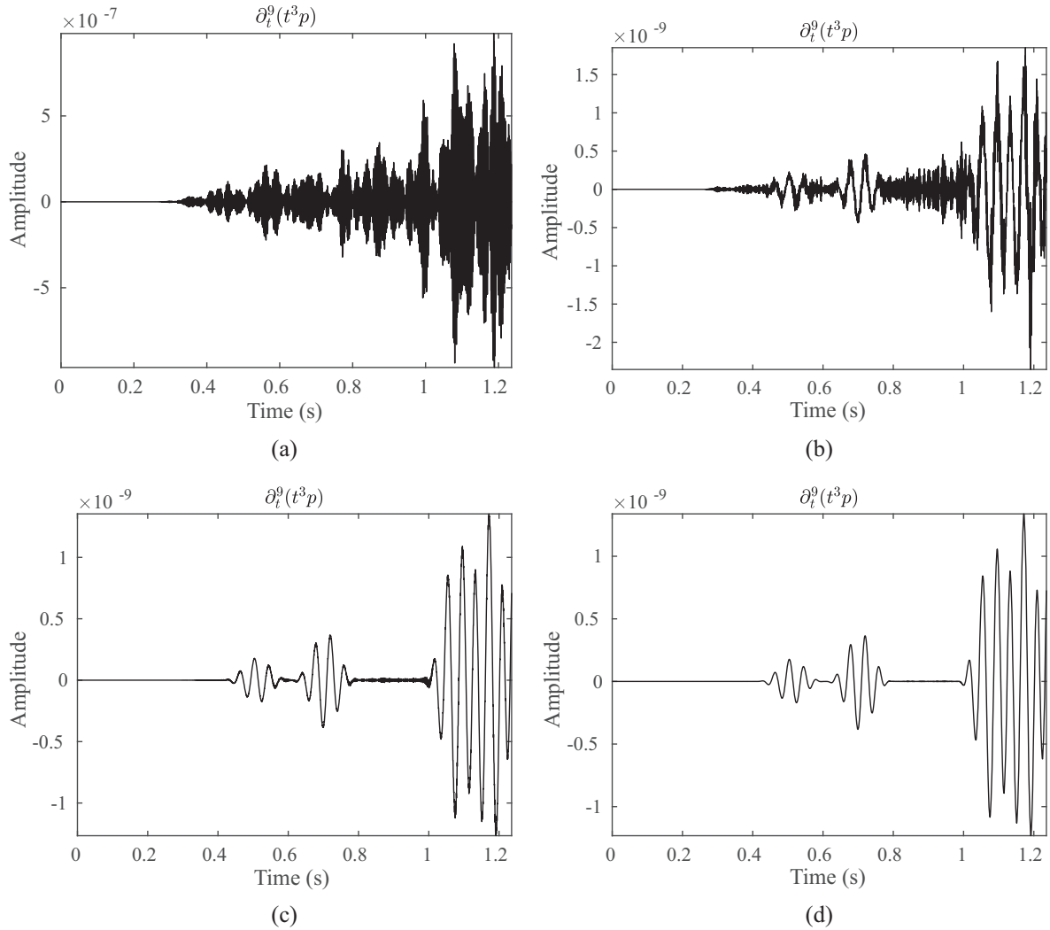
FIGURE 6 Effect of the number of extra stencil points on the removal of numerical noise for the approximation of the term \partial_t^{2k+\ell} [t^\ell \tilde{u}] with k = 3 and \ell = 3 . Half the number of extra points equals 0 (a), 2 (b), 3 (c) or 4 (d).
