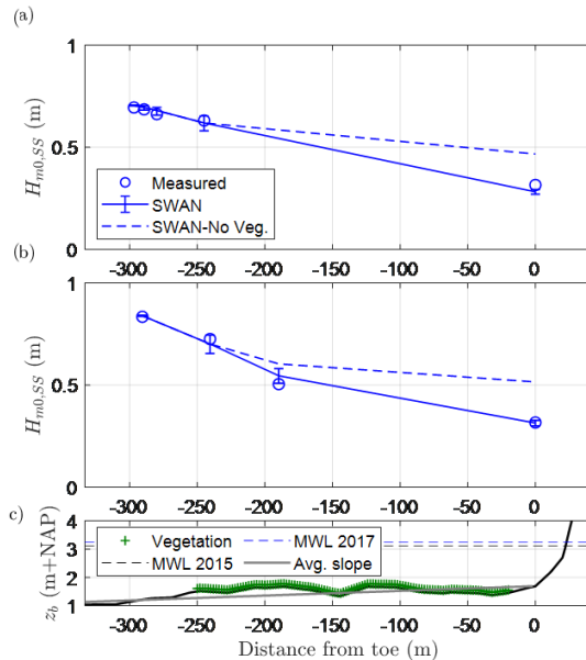
Figure 6. Comparison of measured and modelled significant wave heights in the SS bands ( H_{m0,SS} ) at the peaks of the (a) January 2015 and (b) January 2017 storms at Uithuizerwad (see Fig. 5 for gauge locations). Error bars represent the uncertainty in the estimates based on the standard deviation of Eq. (4). Panel (c) shows the bed level and vegetated cover. MWL: mean water level (at the peak of the storm).
